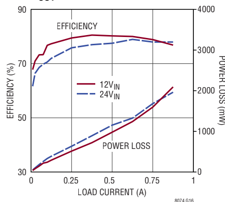
Efficiency and Power Loss, V_{OUT} = -8V
