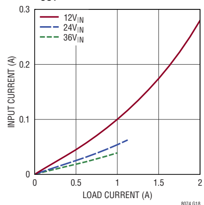
Input vs Load Current, V_{OUT} = 0.8V
