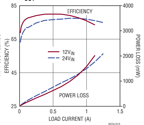
Efficiency and Power Loss, V_{OUT} = -5V
