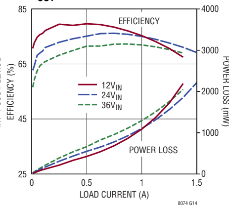
Efficiency and Power Loss, V_{OUT} = -3.3V
