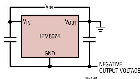
Figure 1. The LTM8074 Can Be Used to Generate a Negative Voltage
