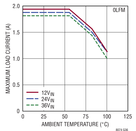
Derating, V_{OUT} = 1\text{V} , DC2753A Demo Board
