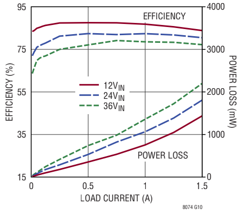
Efficiency and Power Loss, V_{OUT} = 5V
