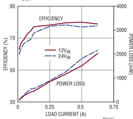
Efficiency and Power Loss, V_{OUT} = -12V
