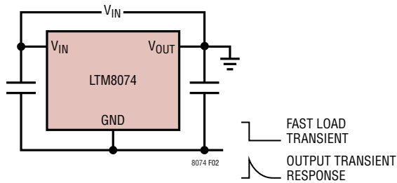
Figure 2. Any Output Voltage Transient Appears on LTM8074 GND
