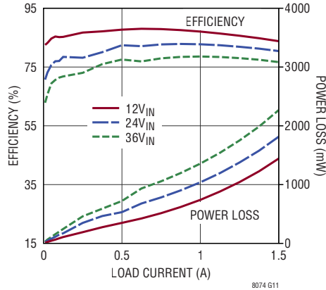
Efficiency and Power Loss, V_{OUT} = 5V , f_{SW} = 2\text{MHz}
