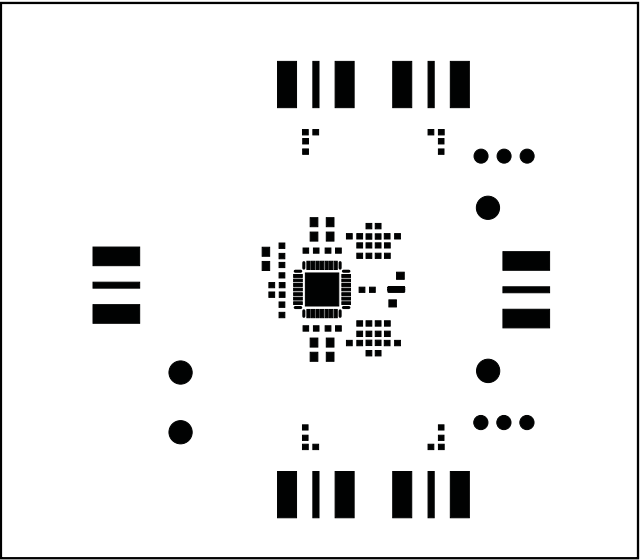
Figure 5. MAX2021 EV Kit PCB Layout—Top Soldermask
