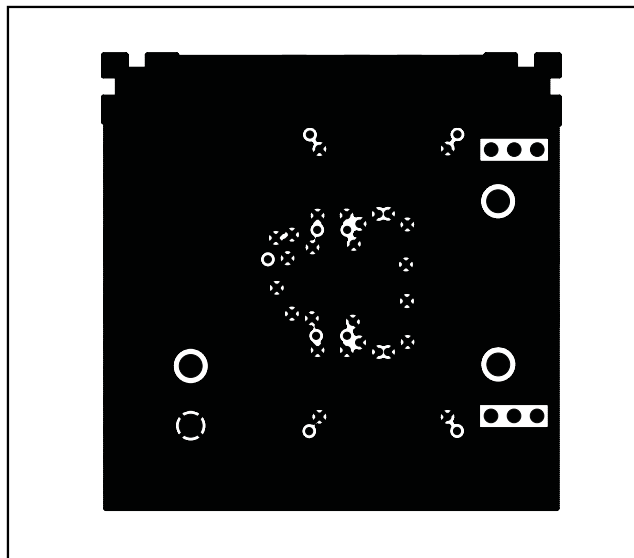
Figure 9. MAX2021 EV Kit PCB Layout—Bottom Layer (Metal)
