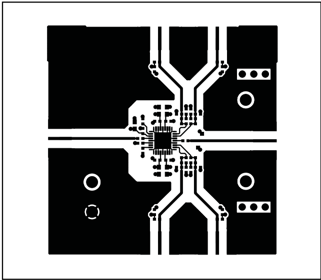
Figure 6. MAX2021 EV Kit PCB Layout—Top Layer Metal
