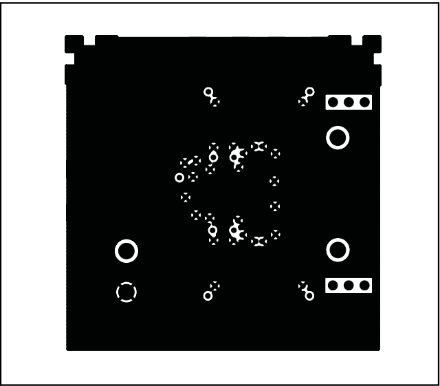
Figure 7. MAX2021 EV Kit PCB Layout—Inner Layer 2 (GND)
