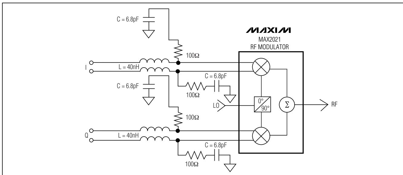
Figure 1. Example Diplexer Network for GSM 900 Applications
