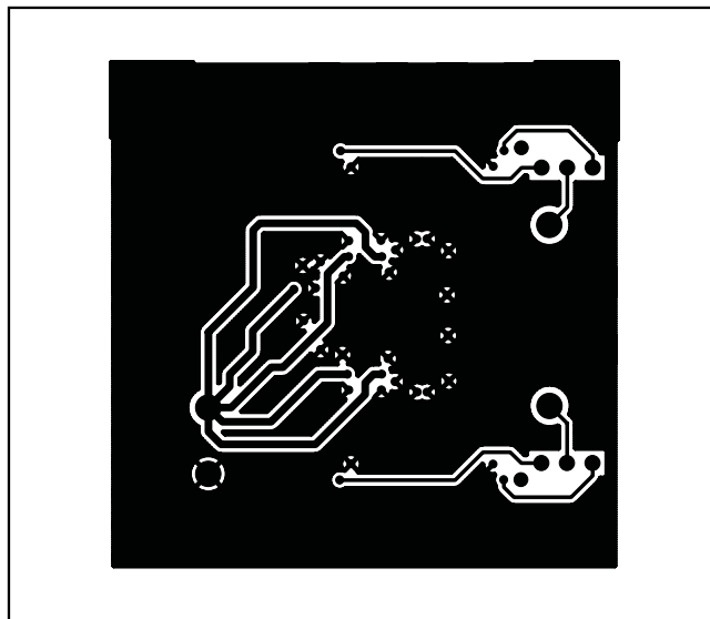
Figure 8. MAX2021 EV Kit PCB Layout—Inner Layer 3 (Routes)
