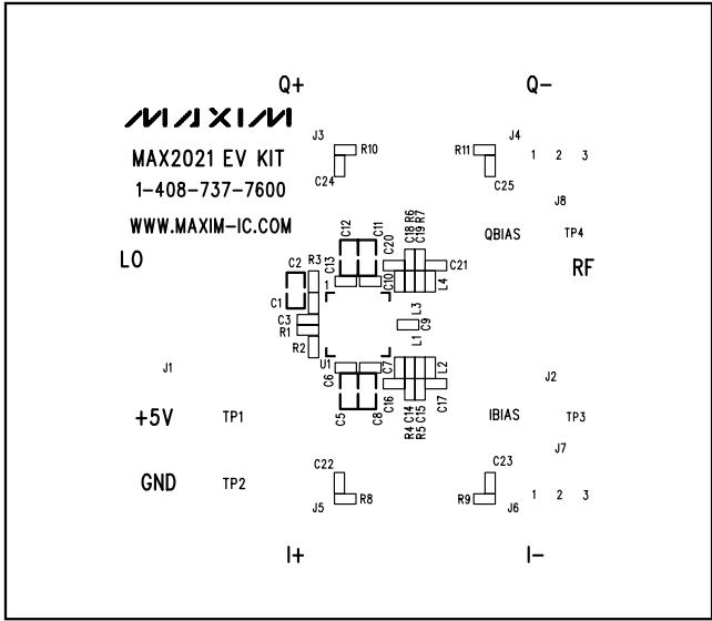
Figure 4. MAX2021 EV Kit PCB Layout—Top Silkscreen
