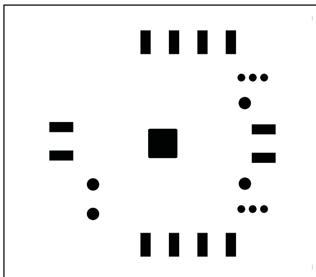
Figure 10. MAX2021 EV Kit PCB Layout—Bottom Soldermask
