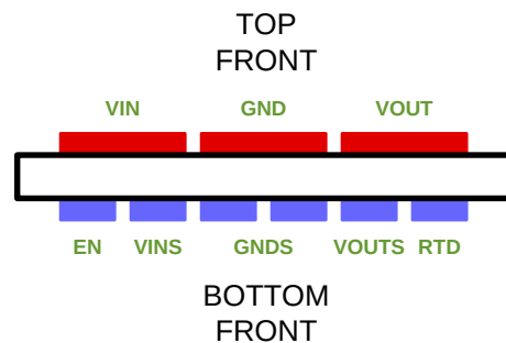
Figure 5. Edge Connector Layout
