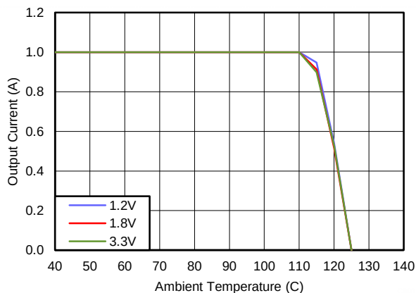
Figure 9. Maximum Output Current vs. Ambient Temperature for LMZ20501 \theta_{JA}=44^{\circ}\text{C/W} , V_{in} = 5\text{V}
