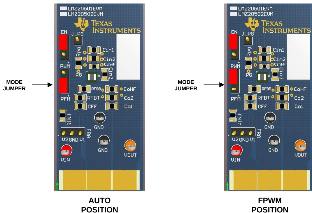
Figure 3. MODE Jumper Configuration
