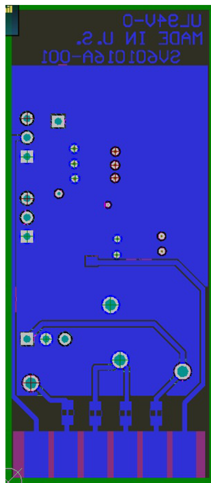
Figure 13. Bottom Metal of EVM
