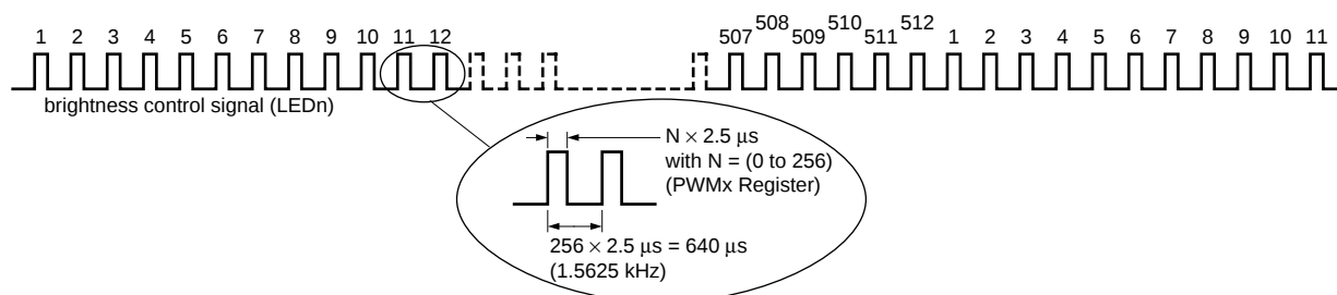
Fig 9. Individual LED brightness control signals
