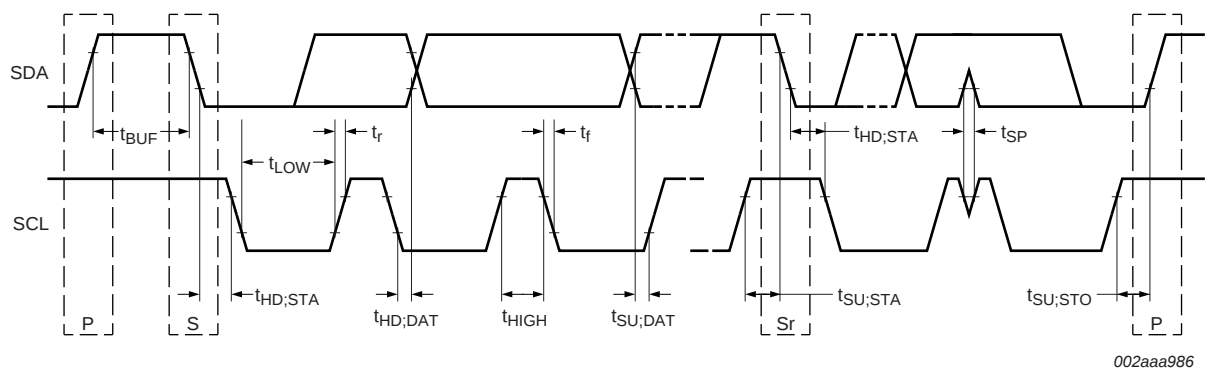
Fig 22. Definition of timing
