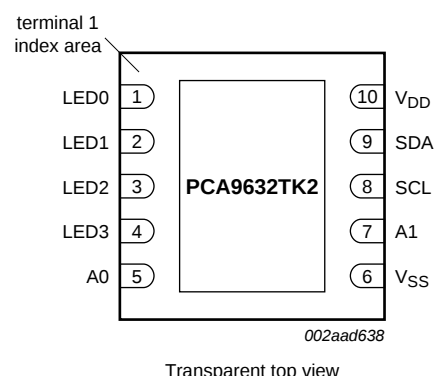
Fig 5. Pin configuration for HVSON10
