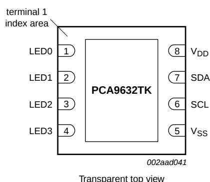
Fig 4. Pin configuration for HVSON8
