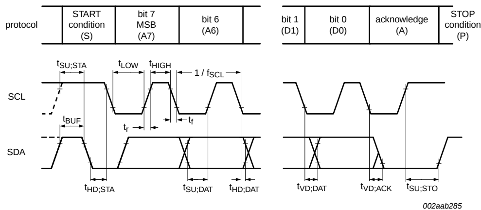
Fig 23. I 2 C-bus timing diagram
