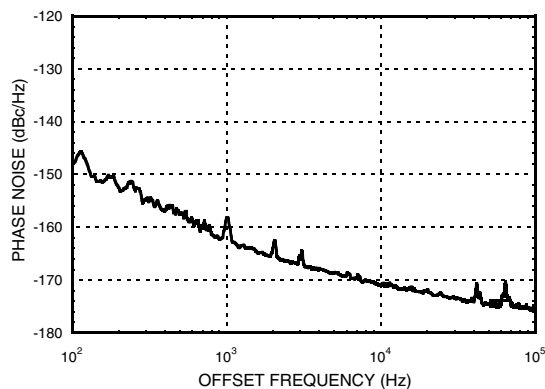
Phase Noise at Pout = +22 dBm @ 3 GHz
