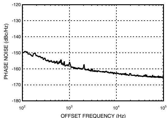
Phase Noise at Pout = +10 dBm @ 3 GHz
