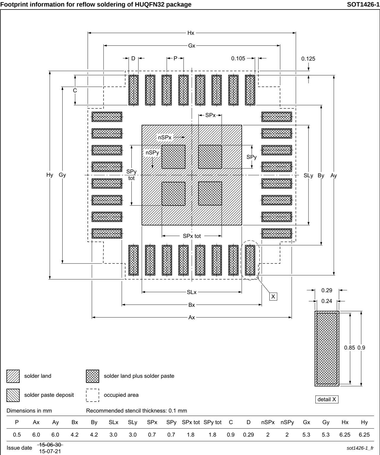
Fig 42. PCB footprint for SOT1426-1 (HUQFN32); reflow soldering
