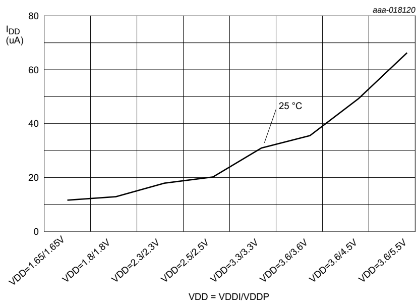
Fig 29. Supply current vs supply voltage
