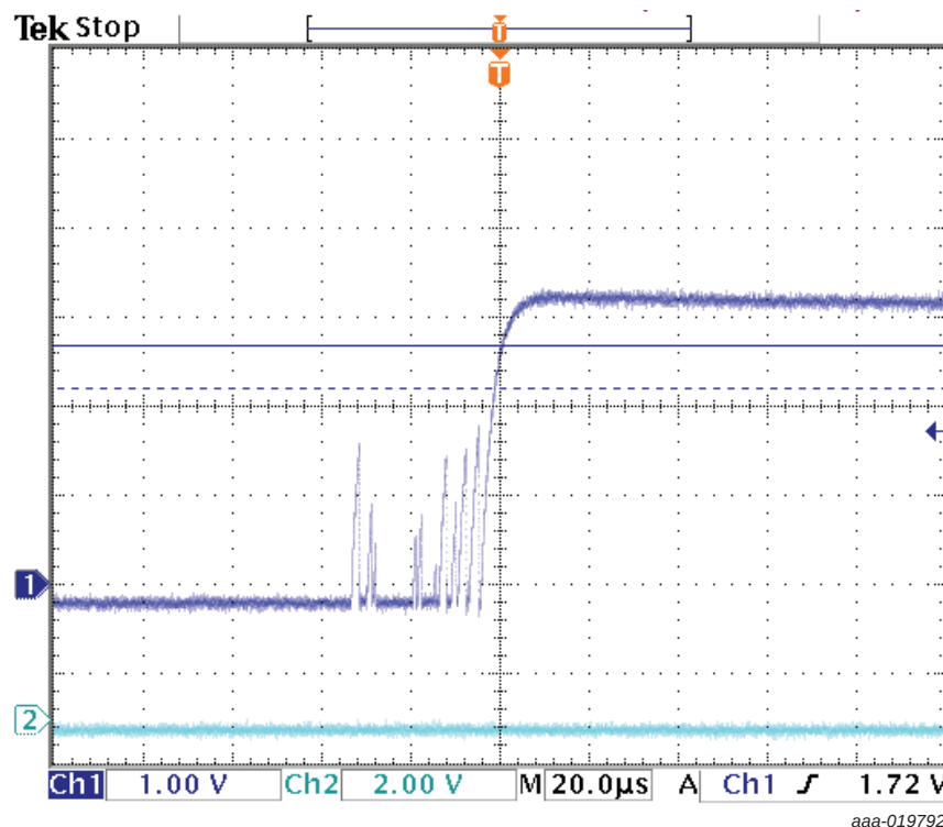
Fig 12. Switch contact bounce
