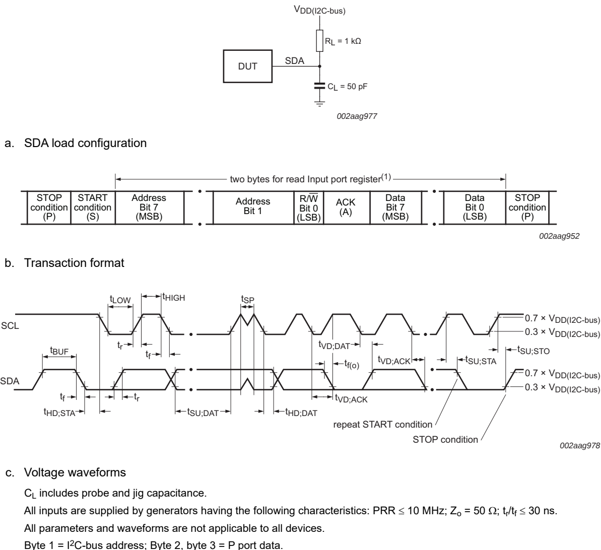
Fig 35. I 2 C-bus interface load circuit and voltage waveforms
