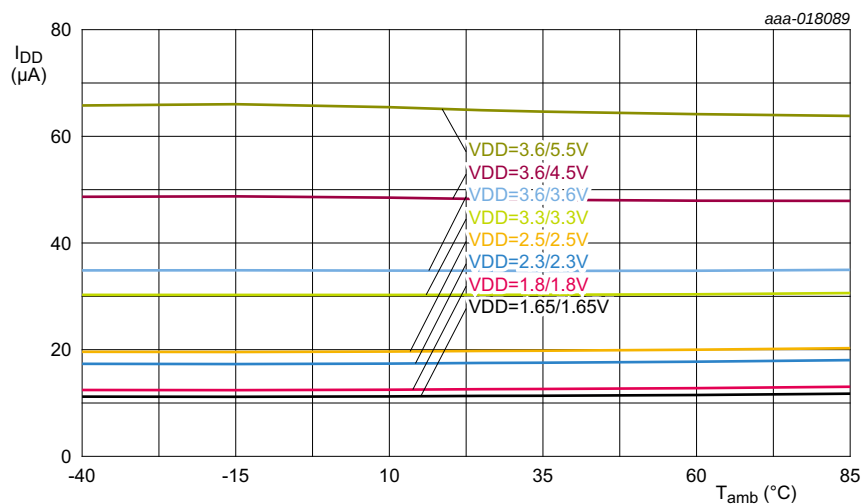
Fig 27. Supply current vs ambient temperature
