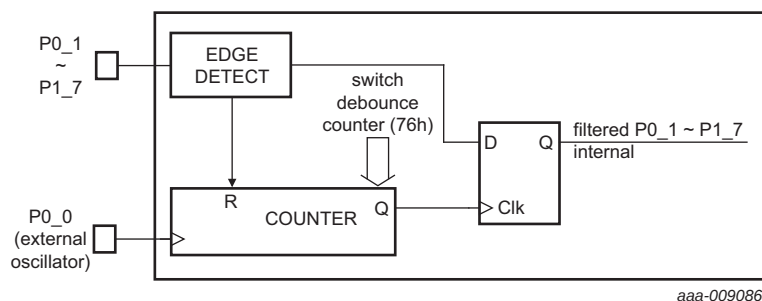
Fig 13. Debouncer block diagram
