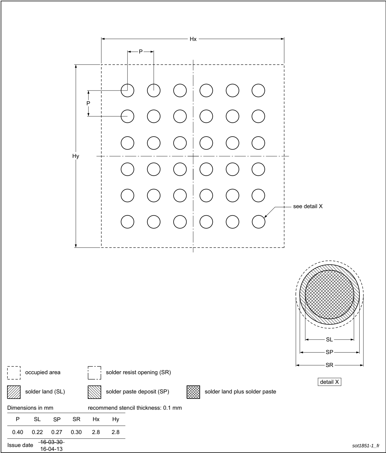
Fig 43. PCB footprint for SOT1851-1 (VFBGA36); reflow soldering
