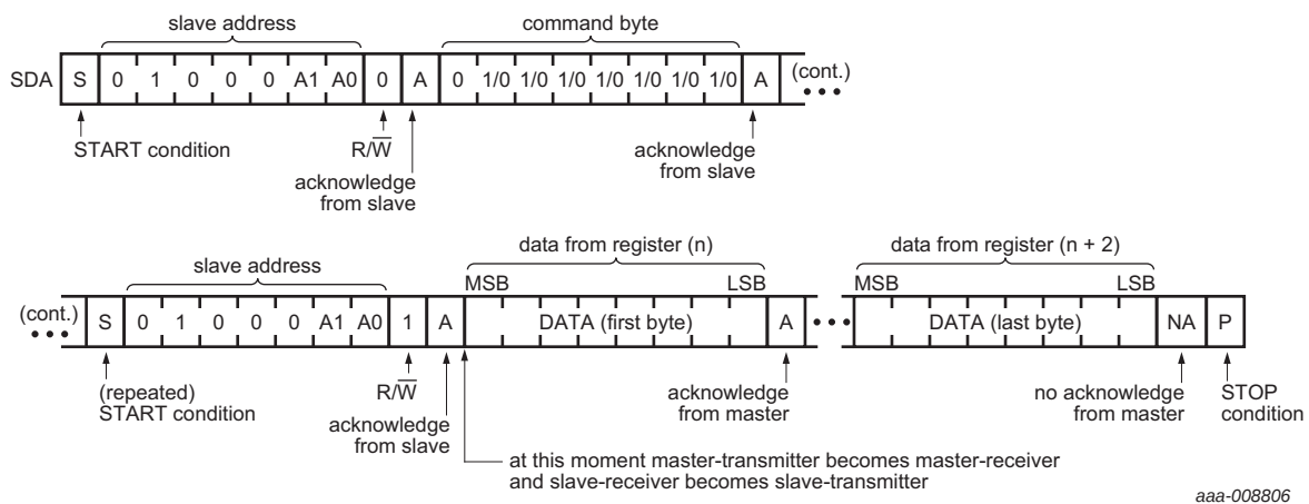
Fig 17. Read from device registers (operate as register triples)
