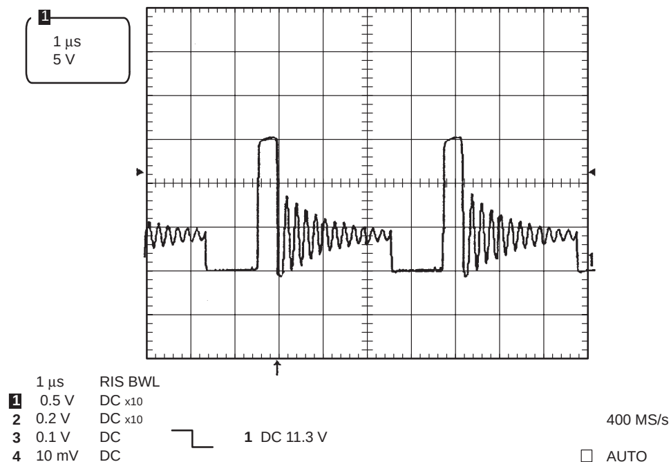
Figure 2–3. SW Waveform
