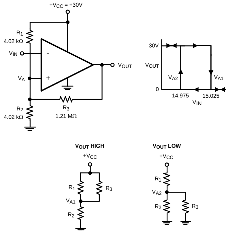
Figure 55. Inverting Comparator with Hysteresis
