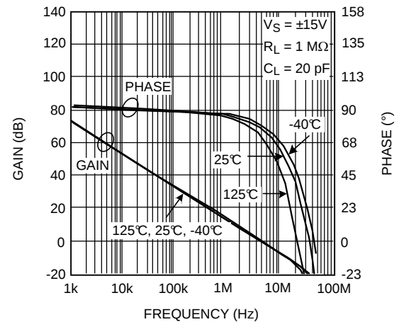
Figure 2. Open Loop Frequency Response
