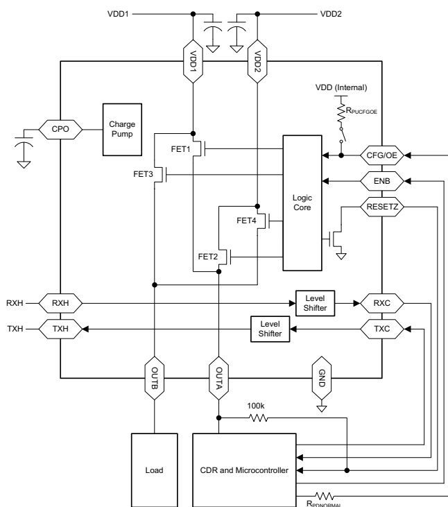
Typical Application
