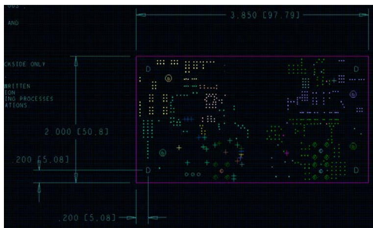
Figure 22. Board Outline
