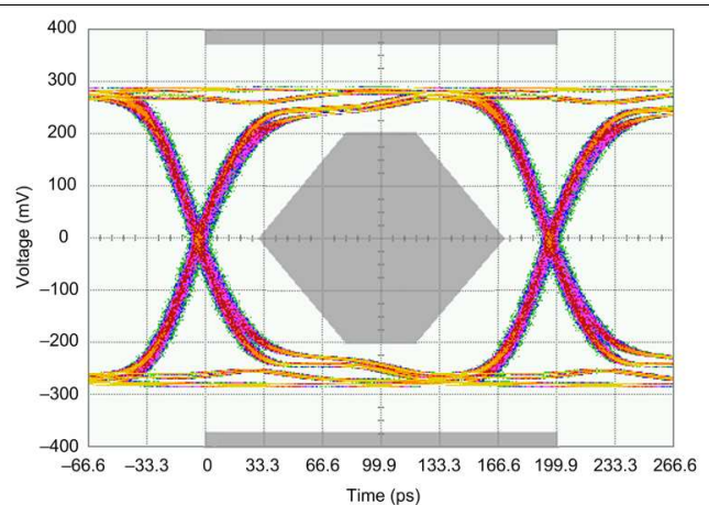
Figure 30. Output Serial Lane Eye Diagram at 5.0 Gb/s
