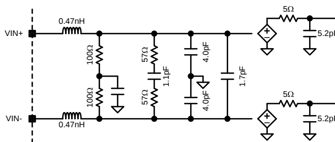
Figure 40. Simplified Analog Input Network Circuit Model
