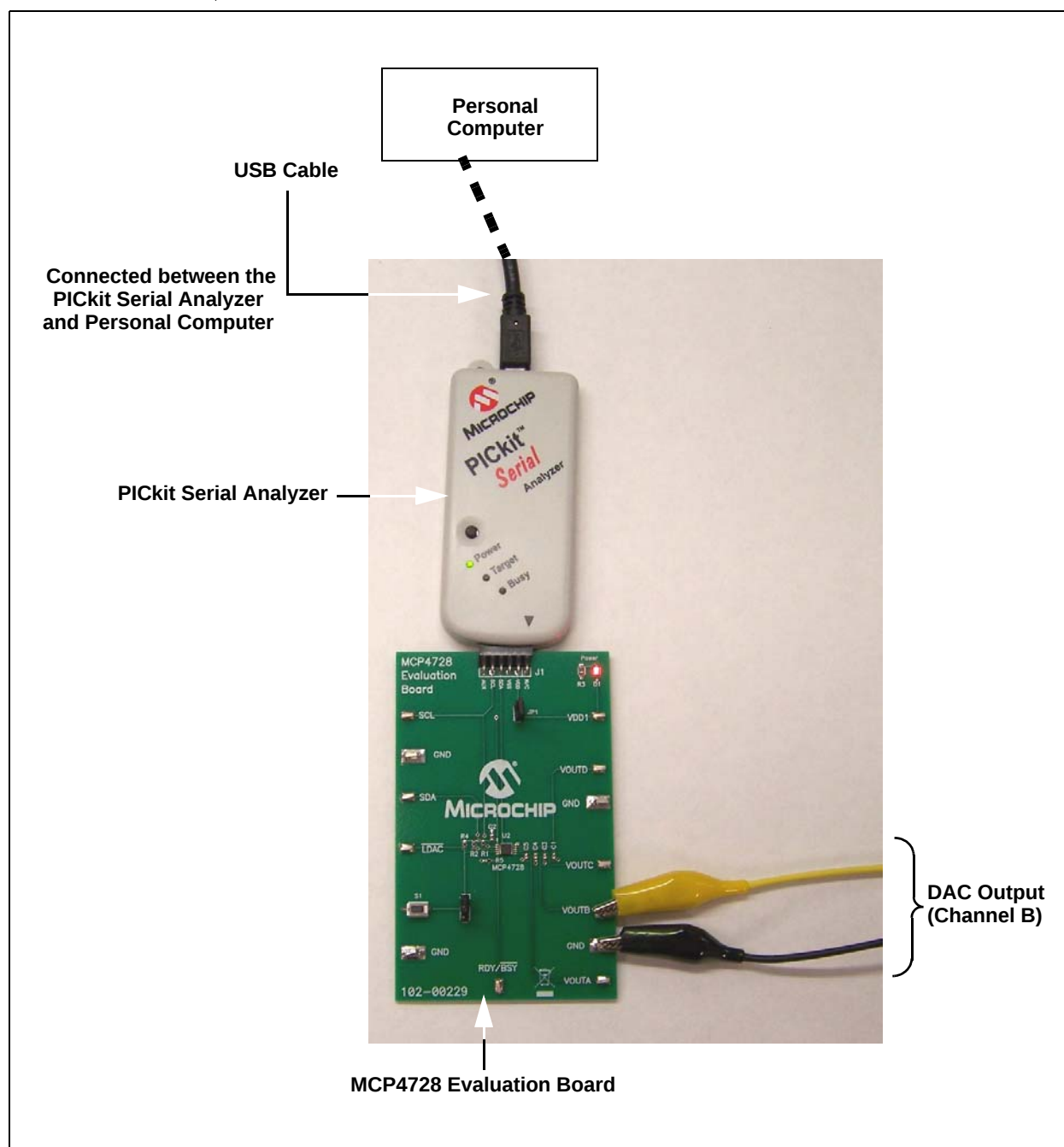
FIGURE 1-2: MCP4728 Evaluation Board with the PICkit Serial Analyzer.
