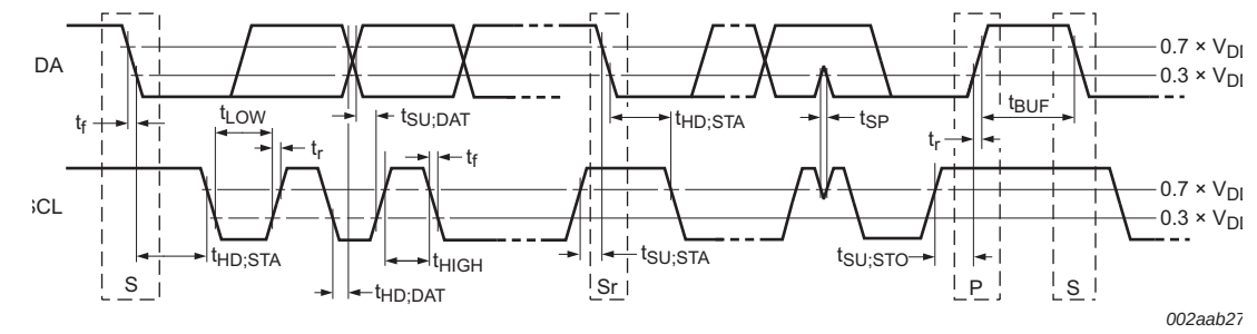
Fig 26. Definition of timing on the I 2 C-bus
