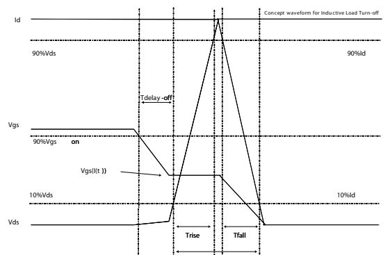
Figure 20: Switching time waveform
