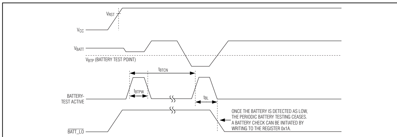
Figure 18. Battery-Test Timing Diagram
