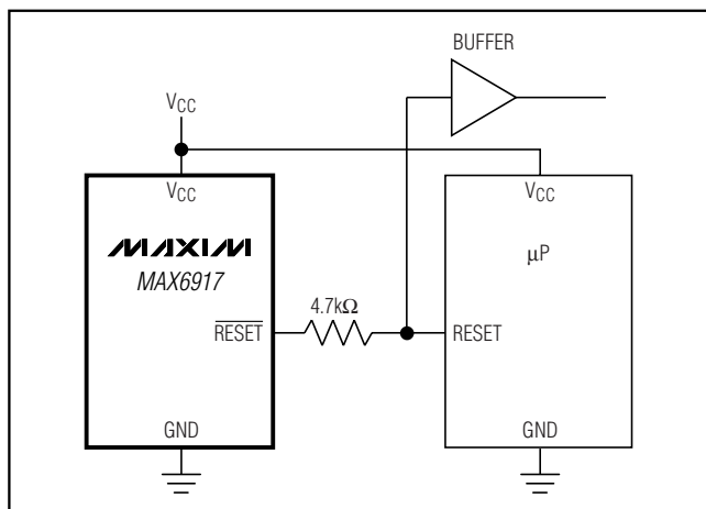
Figure 11. Interfacing to \mu P with Bidirectional Reset I/O
