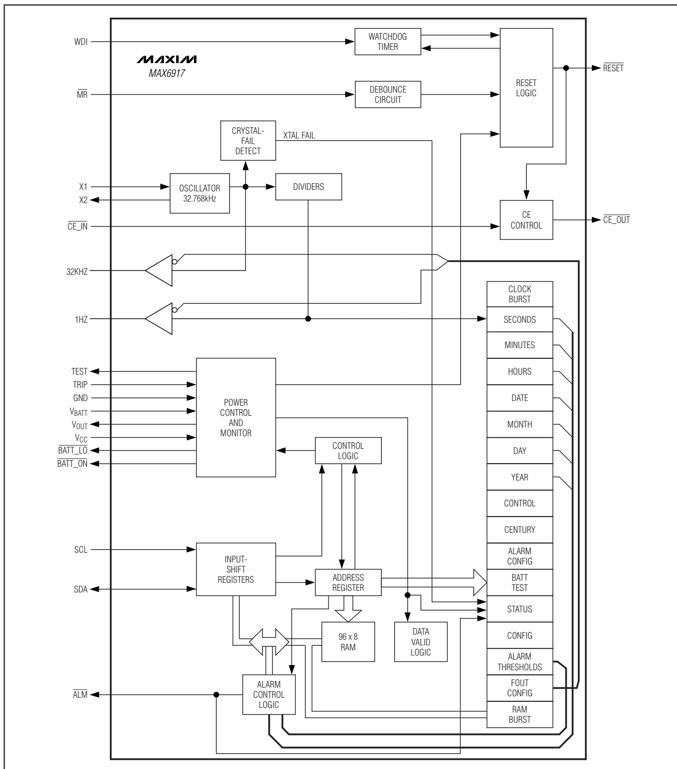
Figure 1. Functional Diagram
