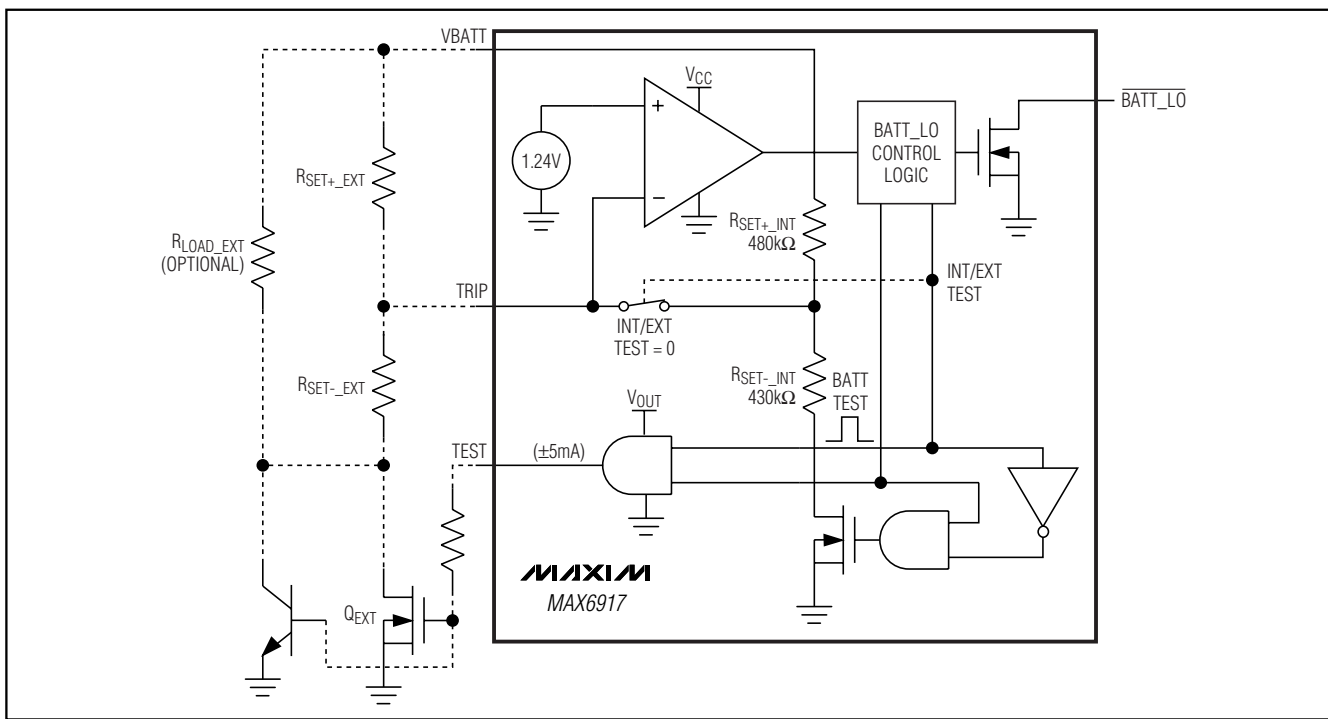
Figure 17. MAX6917 Battery Load and Test Circuit
