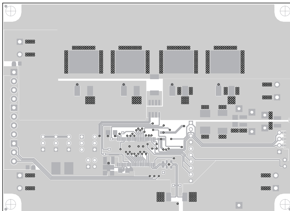
Figure 10. Top Layer
