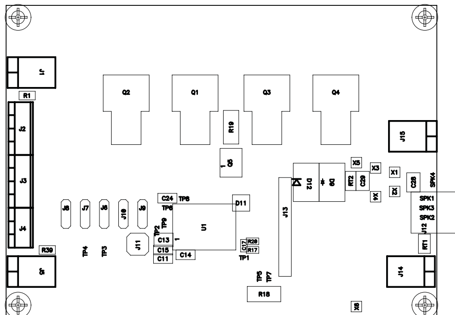
Figure 9. Top Assembly
