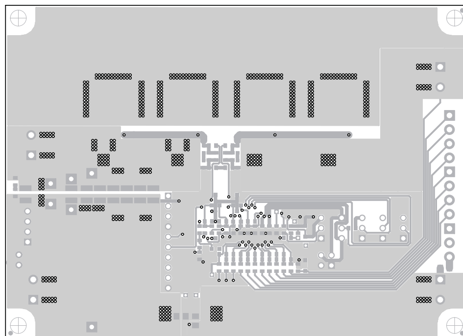
Figure 11. Bottom Layer
