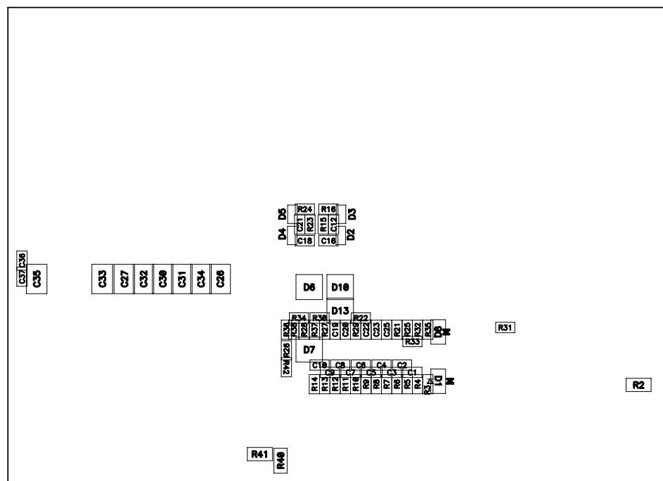
Figure 13. Bottom Assembly
