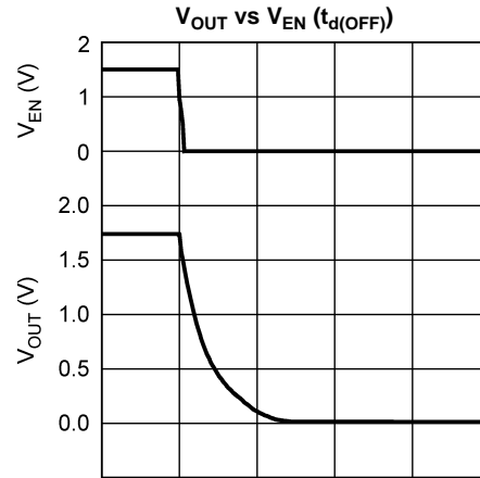
25 \mu\text{s}/\text{DIV} Figure 10.
