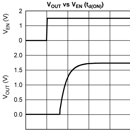
50 \mu\text{s}/\text{DIV} Figure 9.
