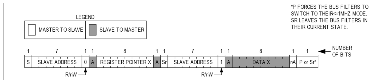
Figure 6. Reading from a single register.
