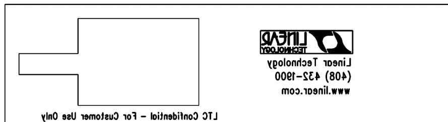
Silkscreen bottom
