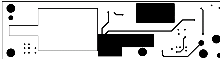
Solder Side
