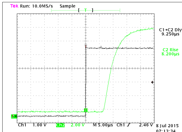
Figure 11. SN65HVDA195-Q1 Dominant to Recessive Prop Delay
