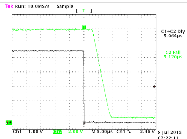
Figure 12. SN65HVDA195-Q1 Recessive to Dominant Prop Delay
