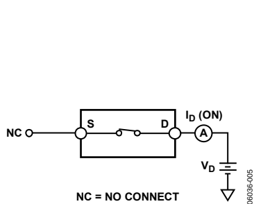
Figure 19. Off Leakage
