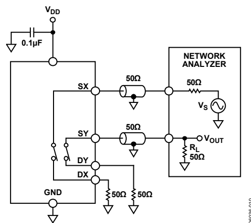
Figure 23. Channel-to-Channel Crosstalk
