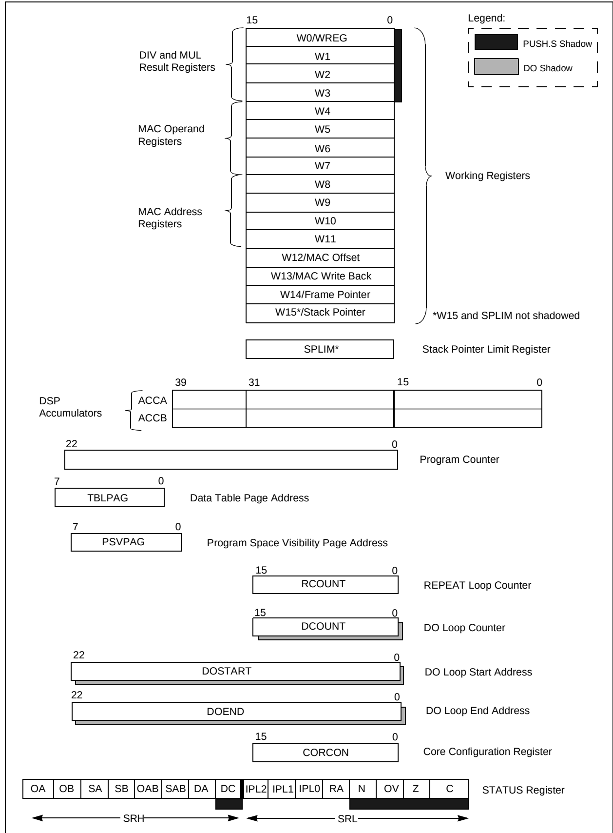
FIGURE 5-2: PROGRAMMER'S MODEL
