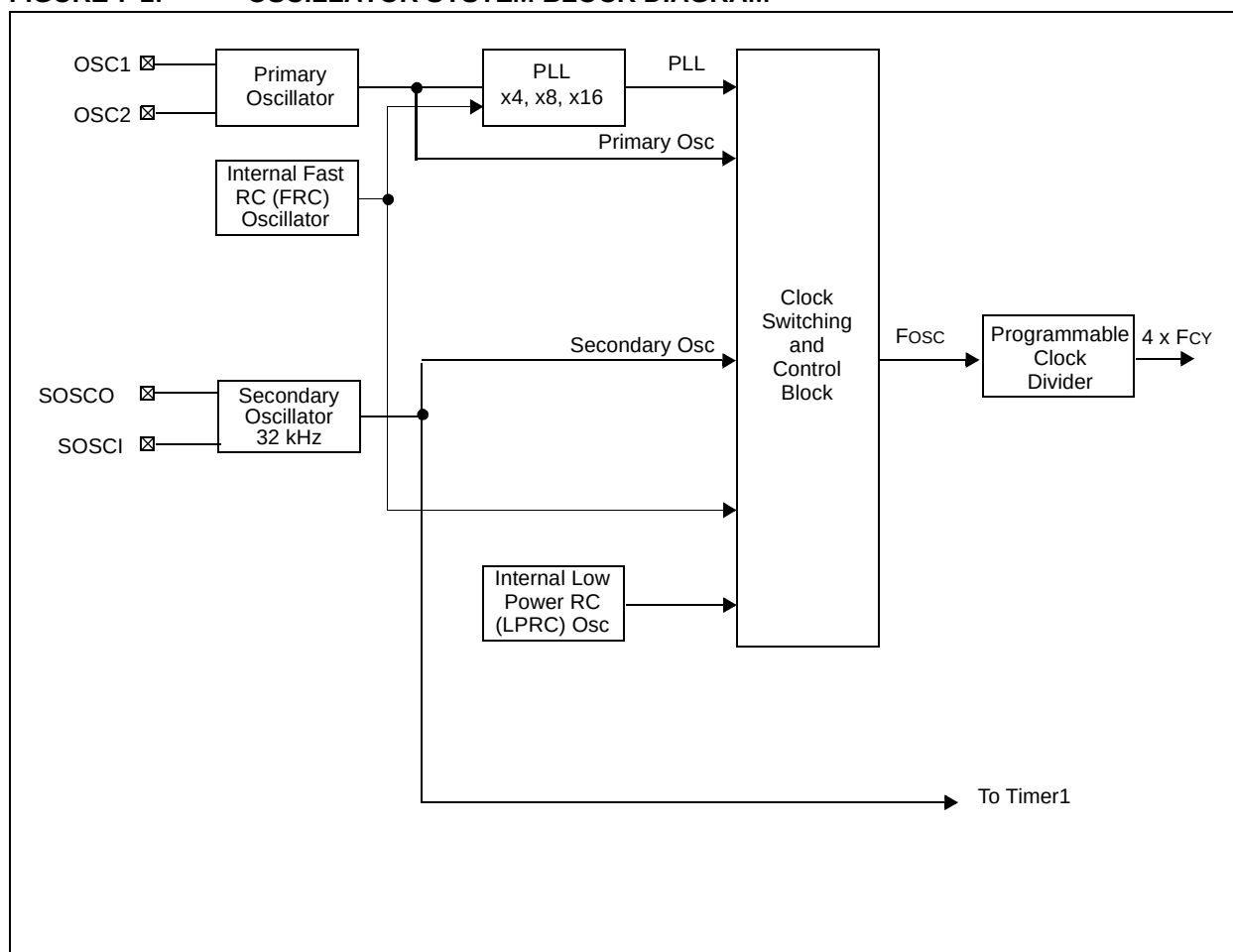
FIGURE 7-1: OSCILLATOR SYSTEM BLOCK DIAGRAM
