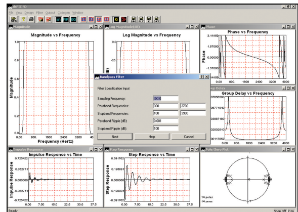
FIGURE 12-2: DIGITAL FILTER DESIGN TOOL INTERFACE
