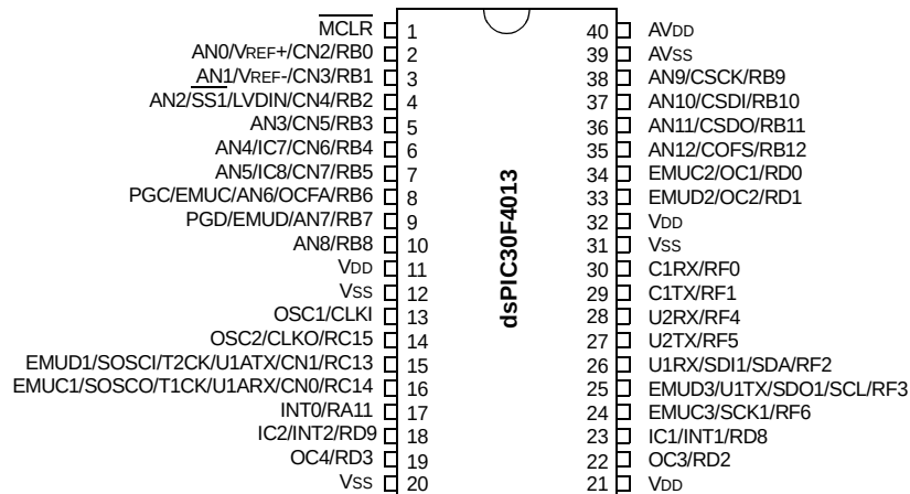
40-Pin PDIP
