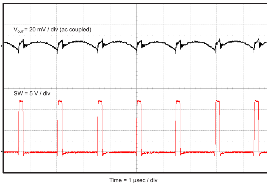
Figure 7. TPS54625EVM-608 Output Voltage Ripple, I_{OUT} = 6.5 A
