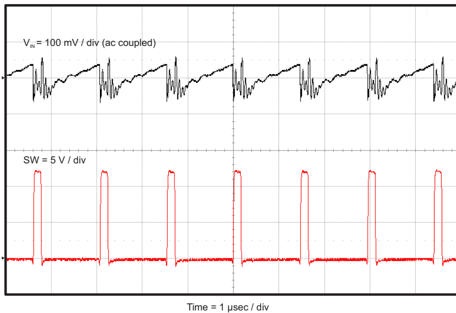
Figure 10. TPS54625EVM-608 Input Voltage Ripple, I_{OUT} = 6.5 A
