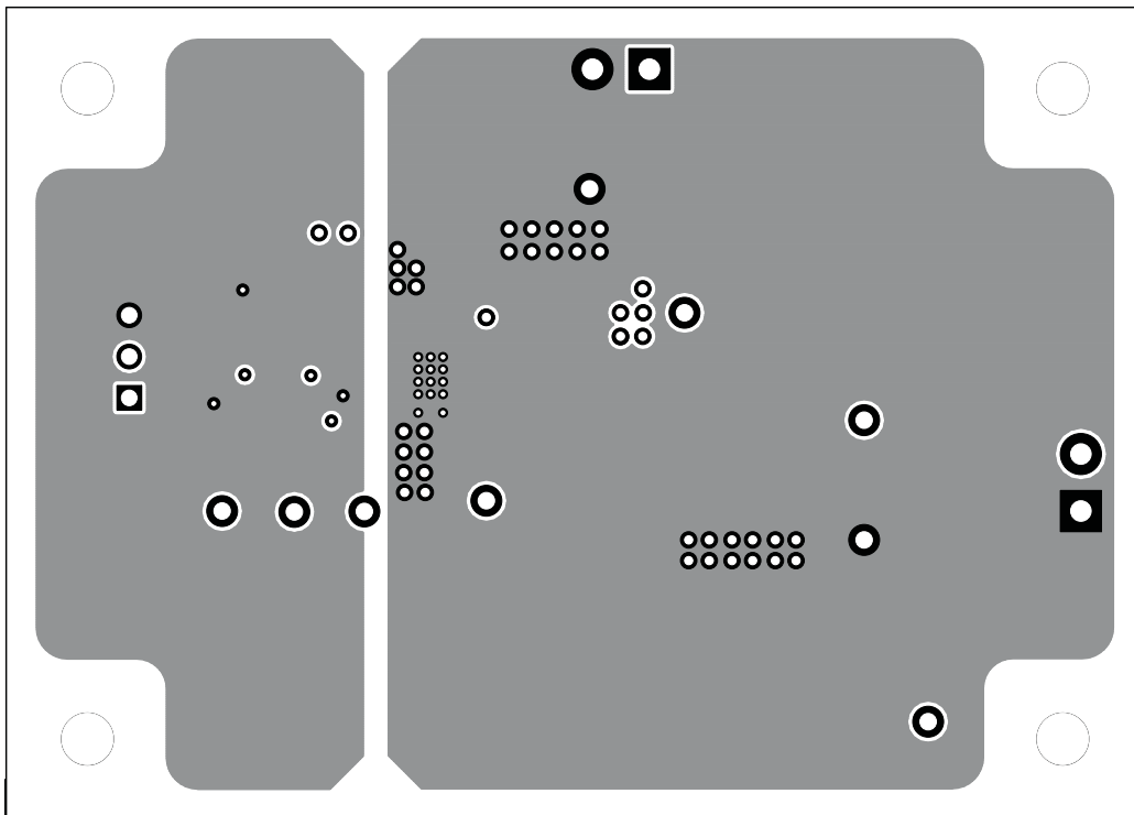
Figure 17. Internal Layer 1
