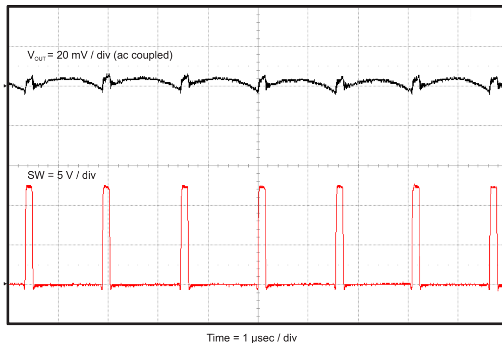
Figure 8. TPS54625EVM-608 Output Voltage Ripple, I_{OUT} = 1 A
