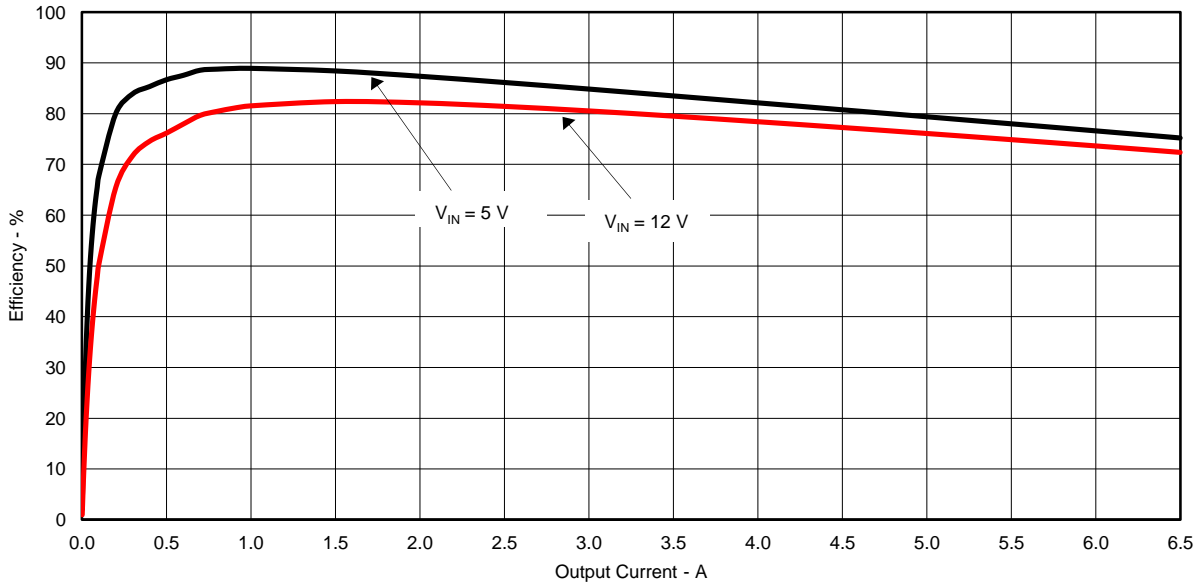
Figure 1. TPS54625EVM-608 Efficiency
