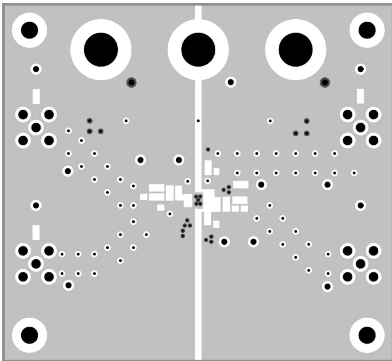
Figure 5. Layer 3 (Power)
