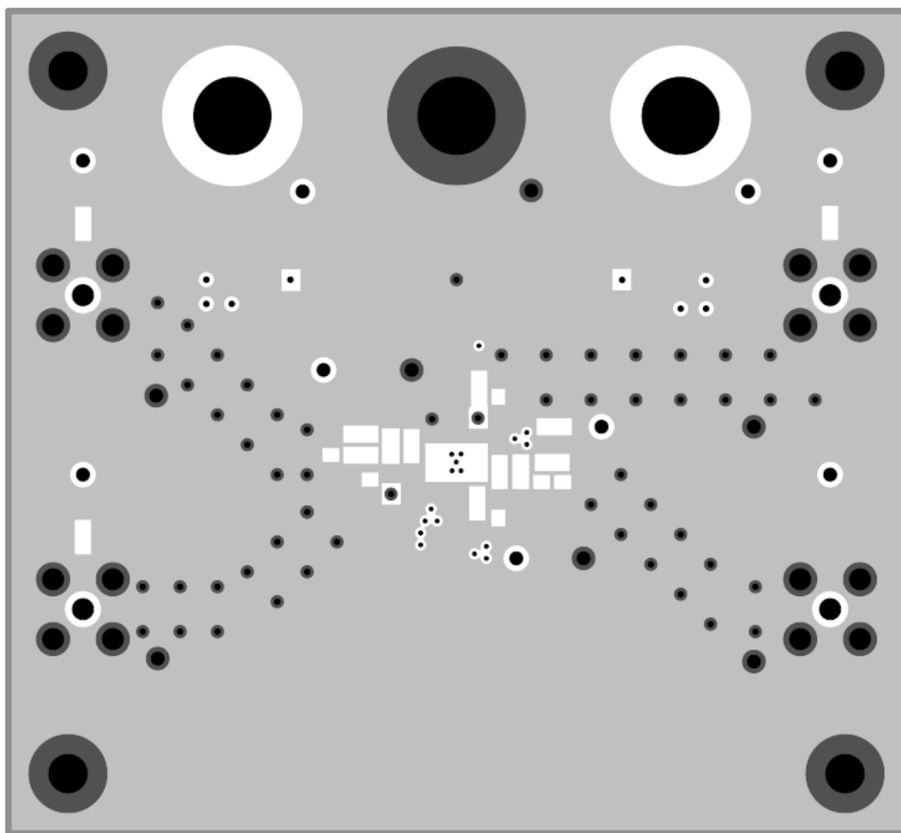
Figure 4. Layer 2 (Ground)
