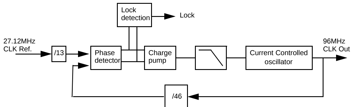
Fig 36. USB PLL
