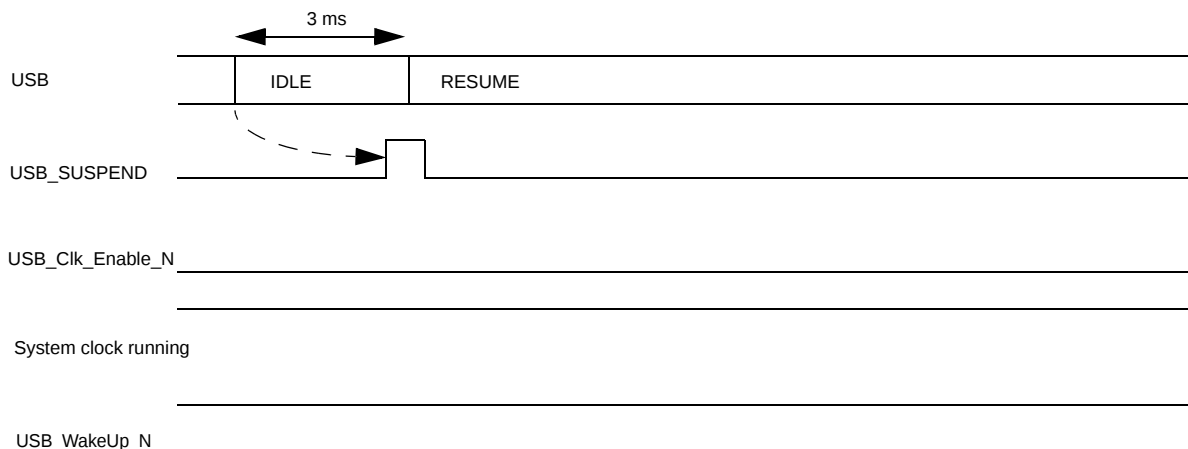
Fig 15. Resume by host / clocks running
