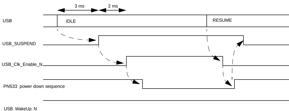
Fig 14. Resume by host/clocks stopped
