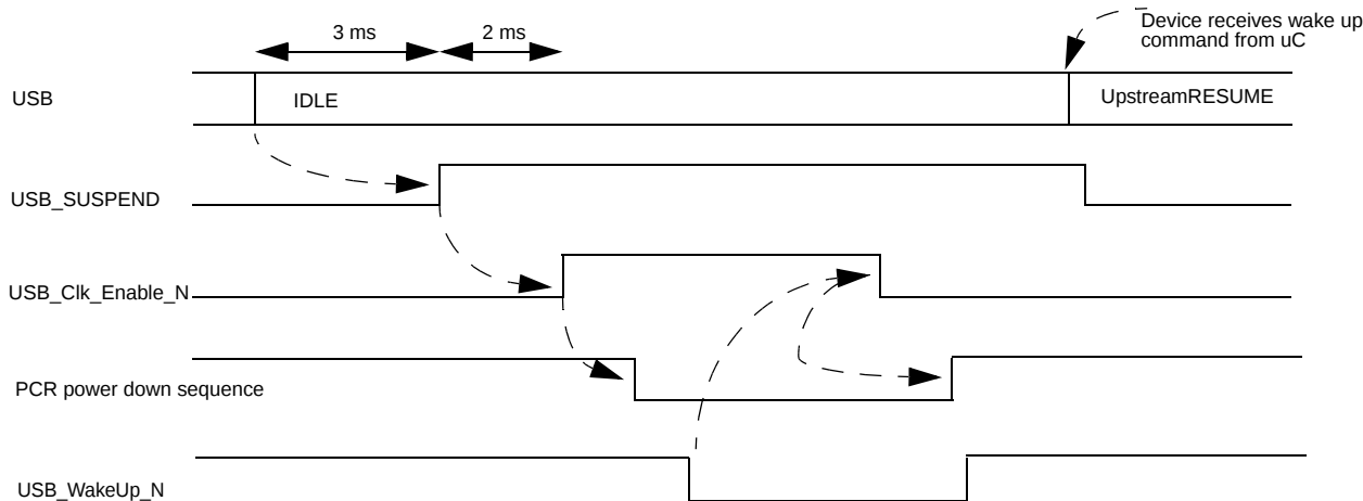
Fig 16. RemoteWakeUp by uC
