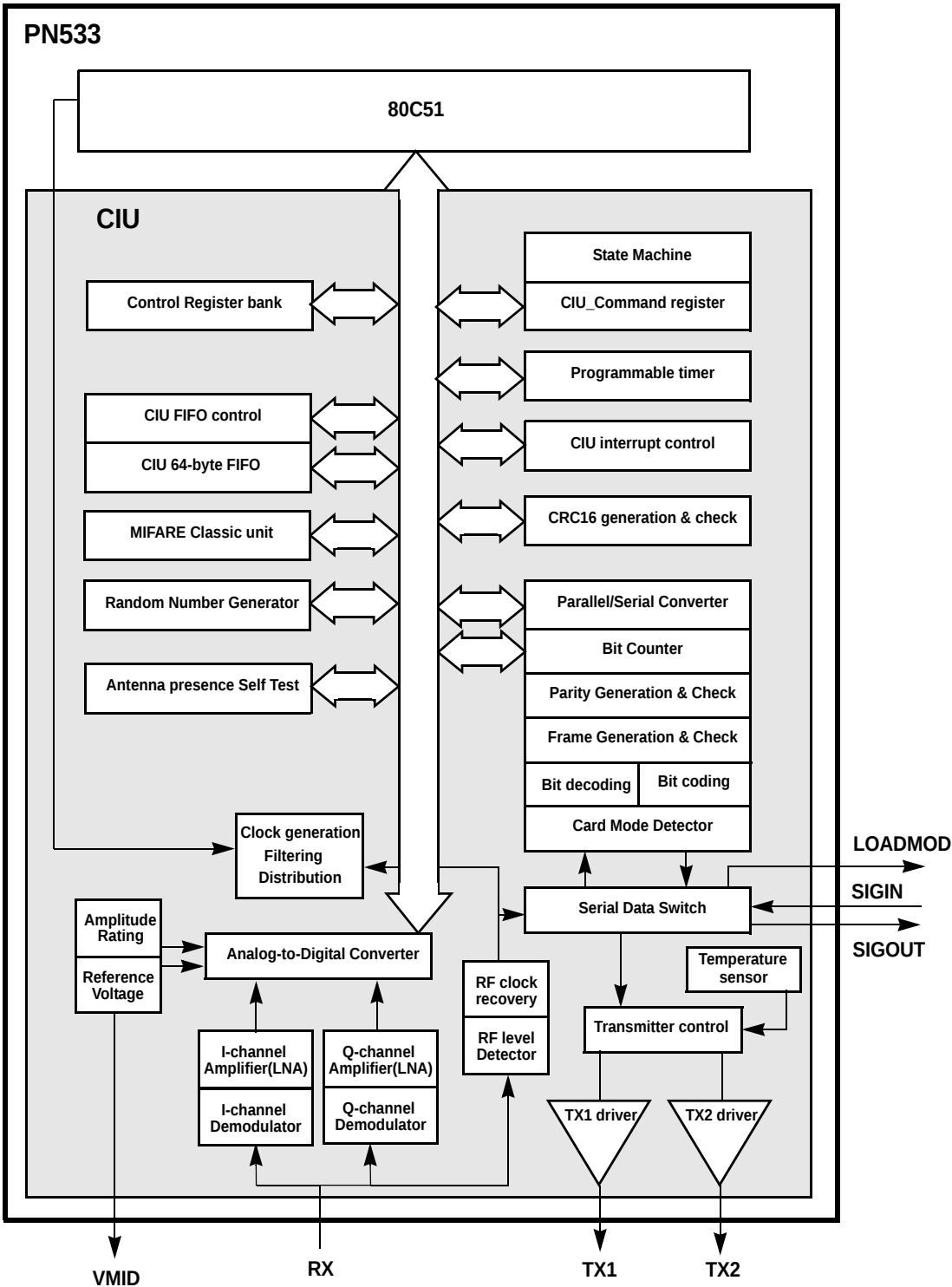
Fig 48. CIU detailed block diagram
