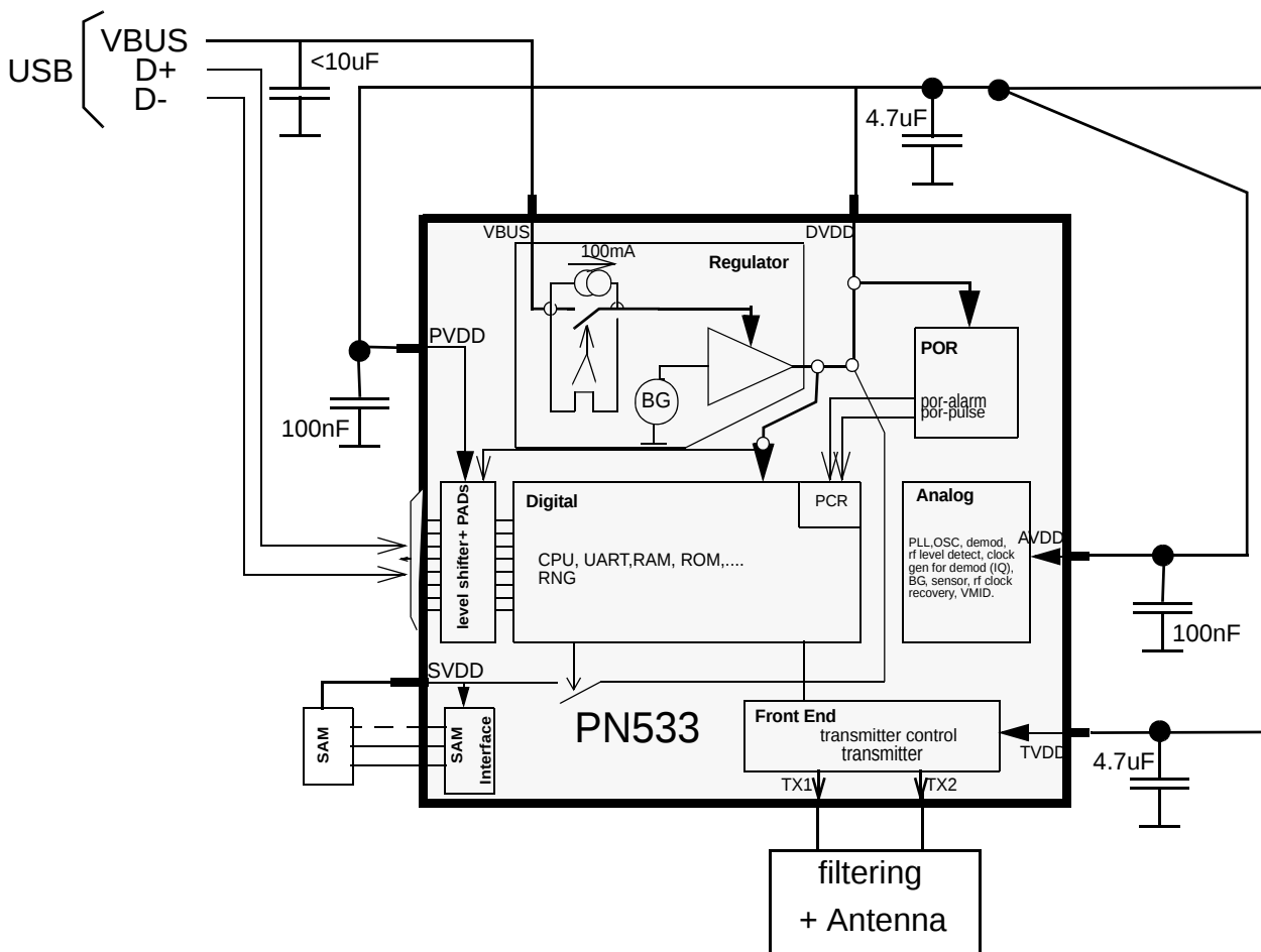
Fig 30. USB bus powered
