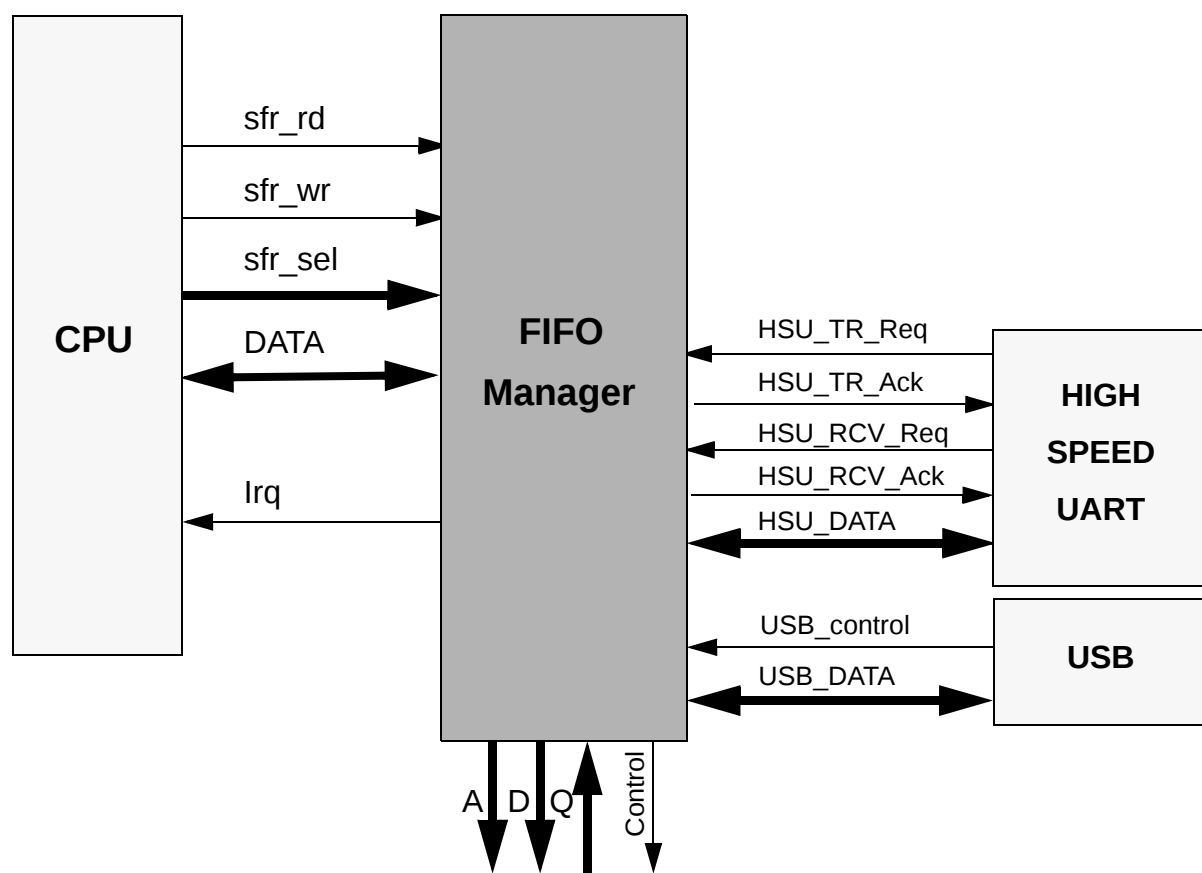
Fig 12. FIFO manager block diagram
