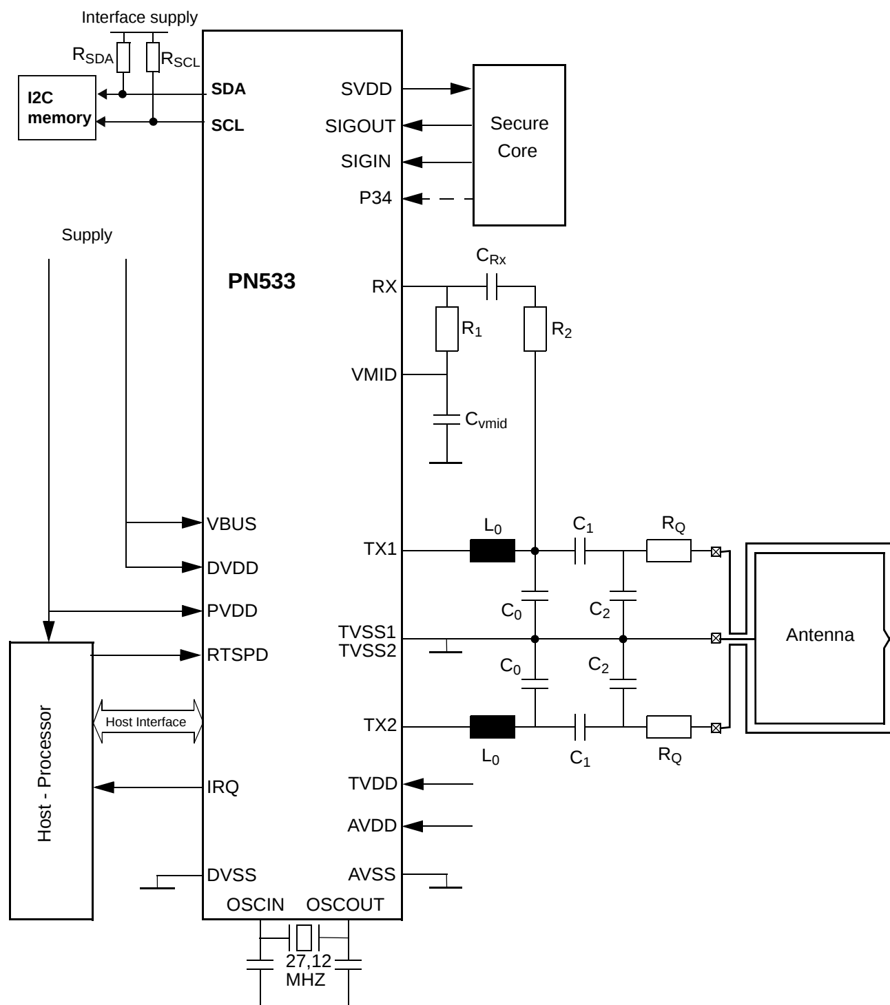
Fig 64. Application diagram of PN533
