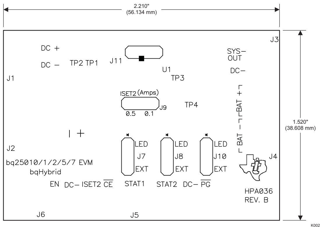
Figure 3-6. Silkscreen
