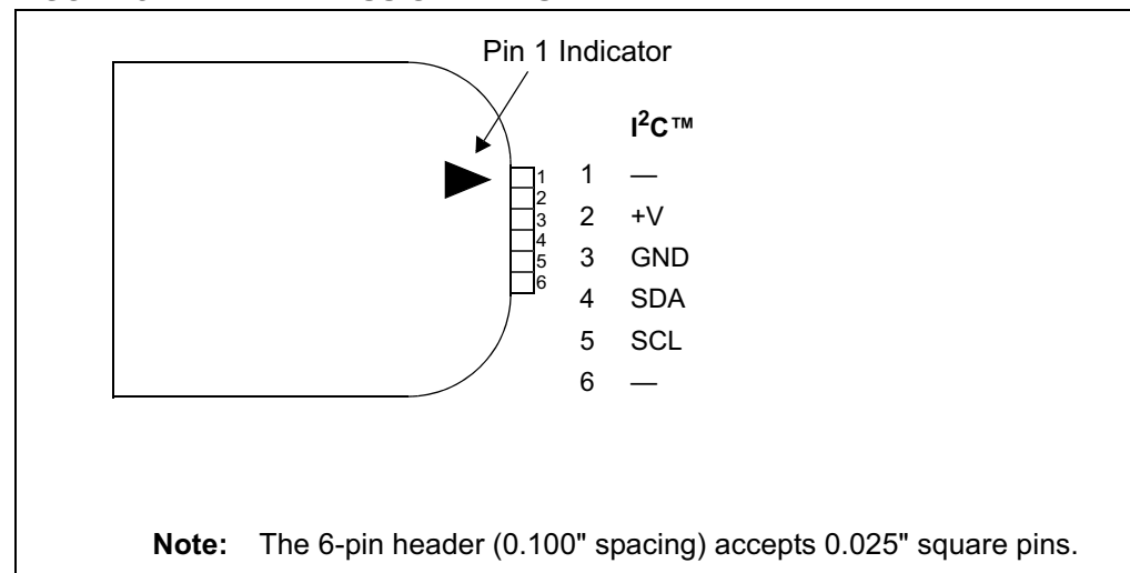
FIGURE 5-1: PIN ASSIGNMENTS
