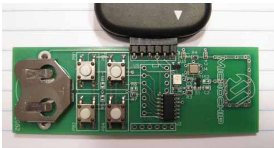
FIGURE 1-3: TRANSMITTER BOARD
