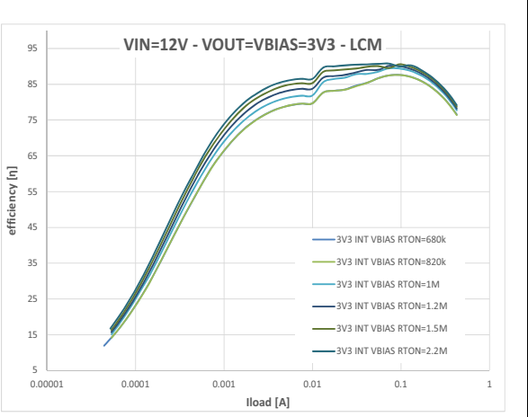
Figure 38. VIN 12 V - VOUT 3.3 V (log scale)
