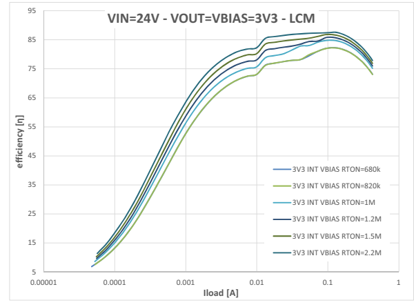
Figure 42. VIN 24V - VOUT 3.3 V (log scale)
