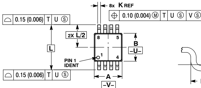
DETAIL E
