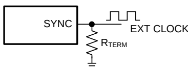
Figure 32. Frequency Synchronization
