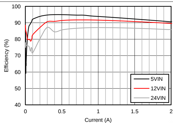
Figure 40. Efficiency at Room Temperature
