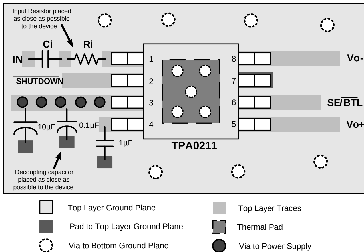
Figure 28. Layout Recommendation
