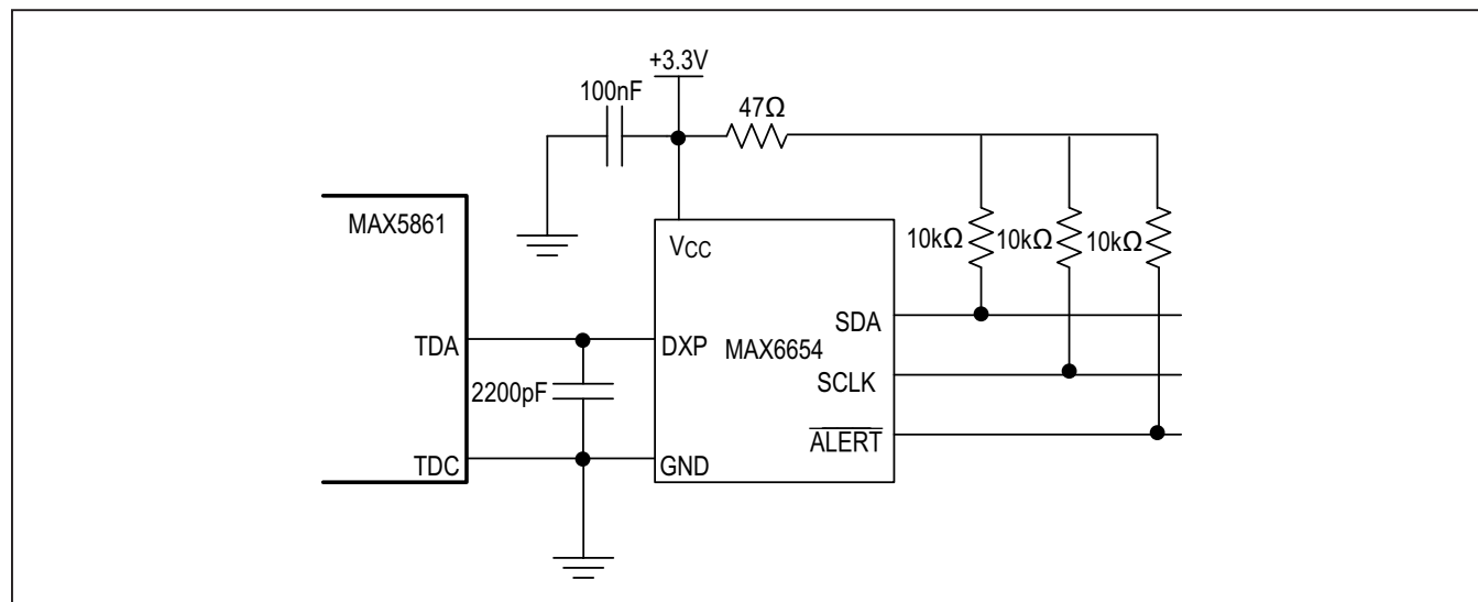
Figure 37. Interfacing to the MAX6654 Temperature Sensor
