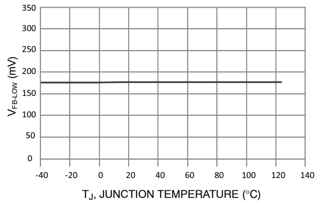
Figure 8. V FB-LOW vs. Temperature
