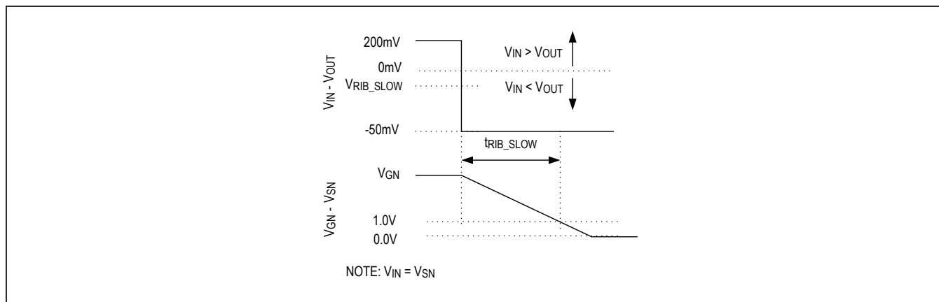
Figure 1. Slow Reverse-Current-Blocking Response Time
