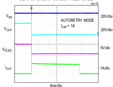
OUTPUT SHORT-CIRCUIT RESPONSE
