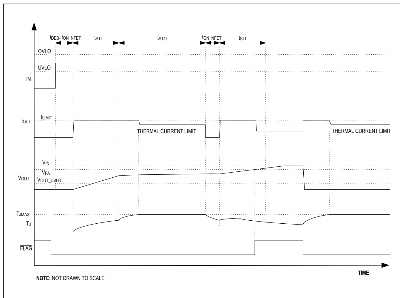
Figure 6. Continuous-Fault Timing Diagram
