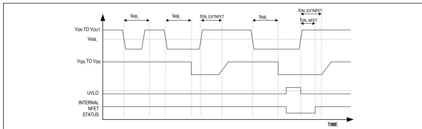
Figure 9. Reverse-Current-Fault Timing Diagram
