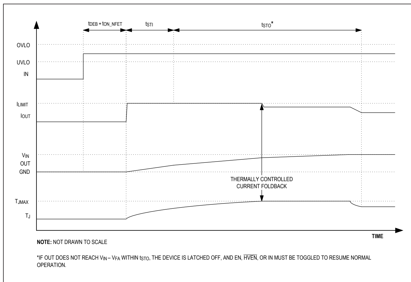
Figure 5. Startup Timing Diagram
