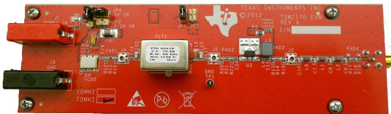
Figure 1. TSW2170EVM Board
