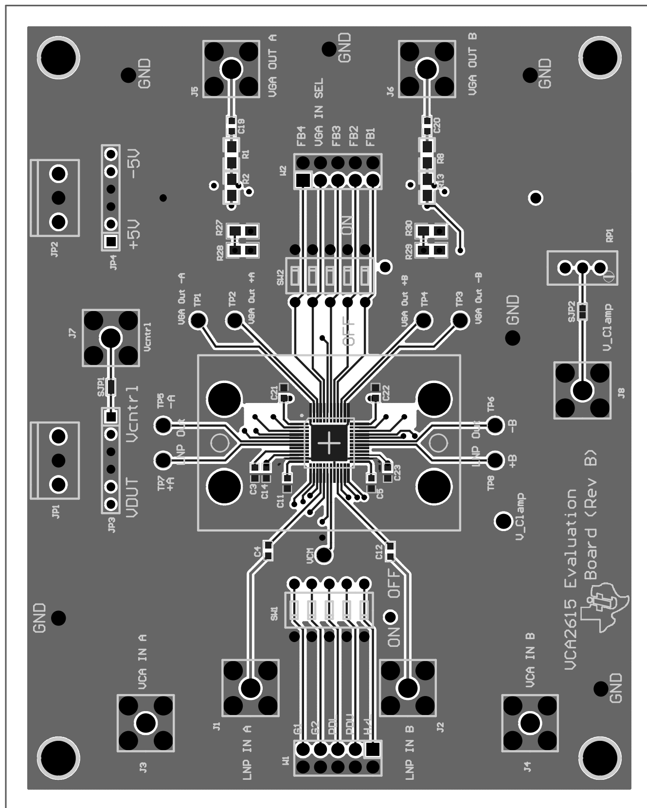
Figure 2. VCA2615EVM PCB Top Layer (Top View)
