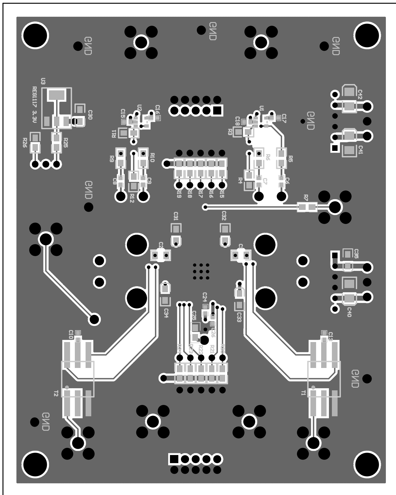
Figure 5. VCA2615EVM PCB Bottom Layer (Bottom View)
