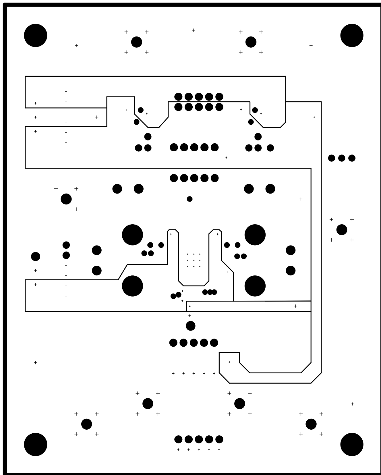
Figure 3. VCA2615EVM PCB Power Layer (Top View)
