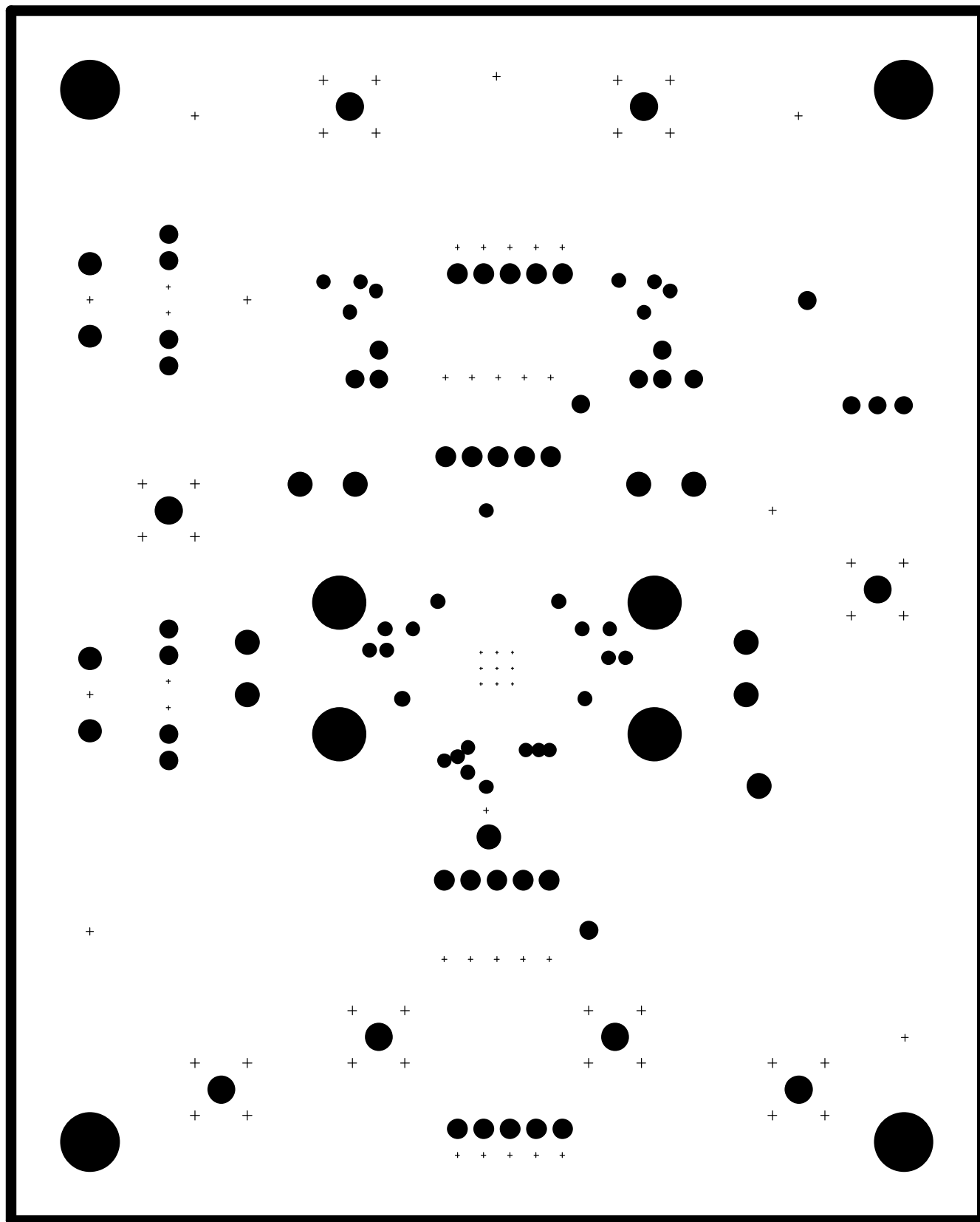
Figure 4. VCA2615EVM PCB Ground Layer (Top View)
