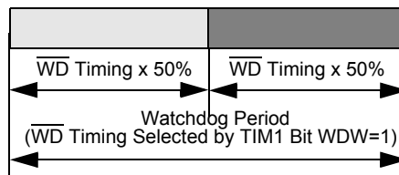
Figure 17. Window Watchdog
