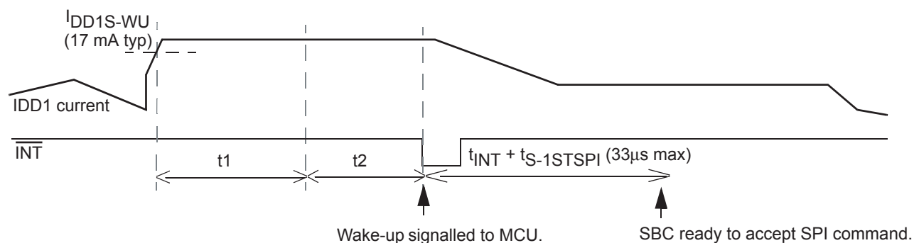
Figure 32. Overcurrent Wake-up
