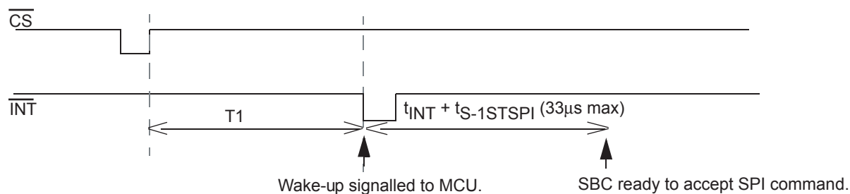
Figure 31. \overline{\text{CS}} Wake-up
