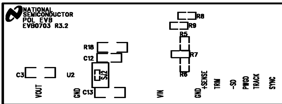
Figure 14. Bottom Silkscreen
