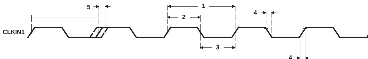
Figure 7-21. CLKIN1 Timing
