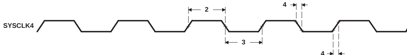
Figure 7-22. SYSCLK4 Timing
