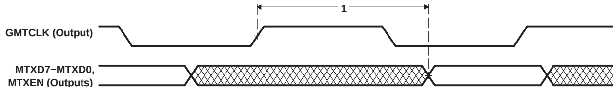
Figure 7-64. EMAC Transmit Interface Timing [GMII Operation]
