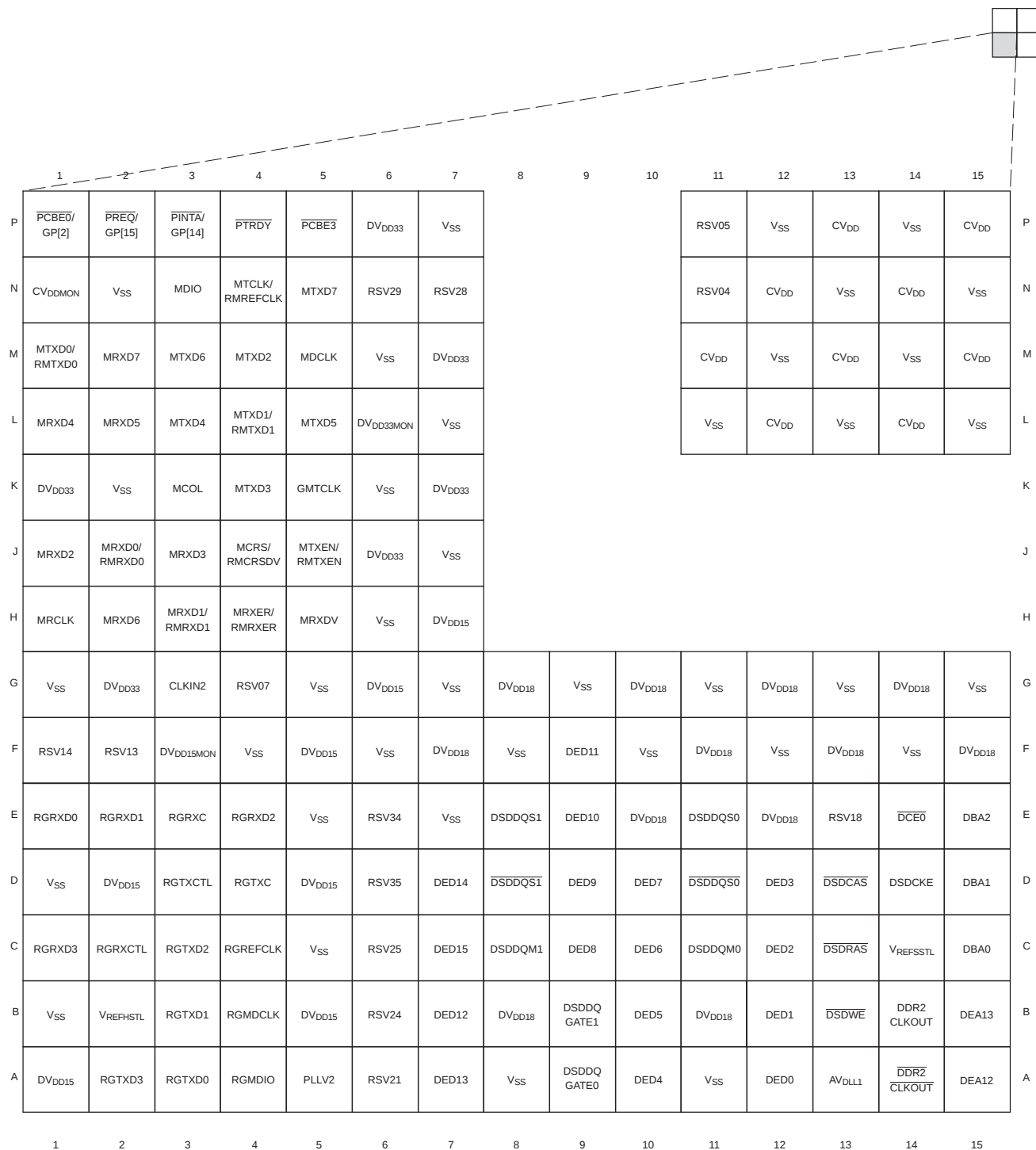
Figure 2-5. C6454 Pin Map (Bottom View) [Quadrant D]
