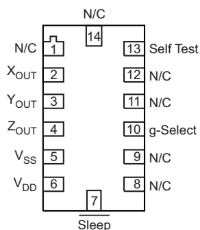
Figure 4. Pinout Description
