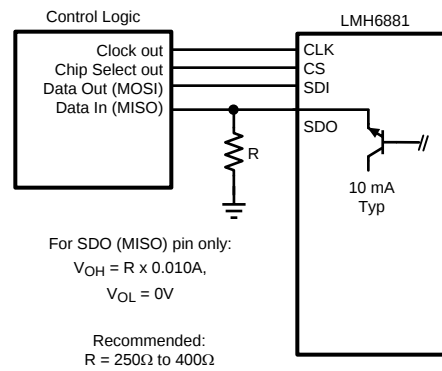
Figure 41. Internal Operation of the SDO Pin
