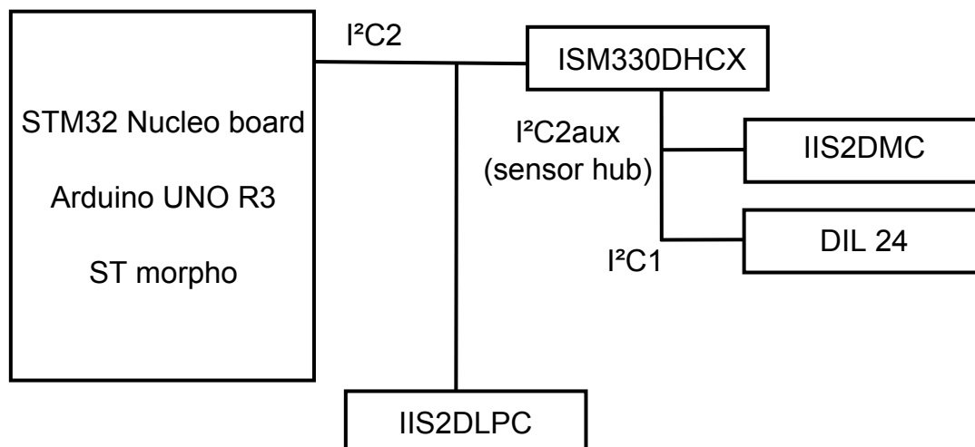
Figure 4. X-NUCLEO-IKS02A1 ISM330DHCX I 2 C sensor hub
