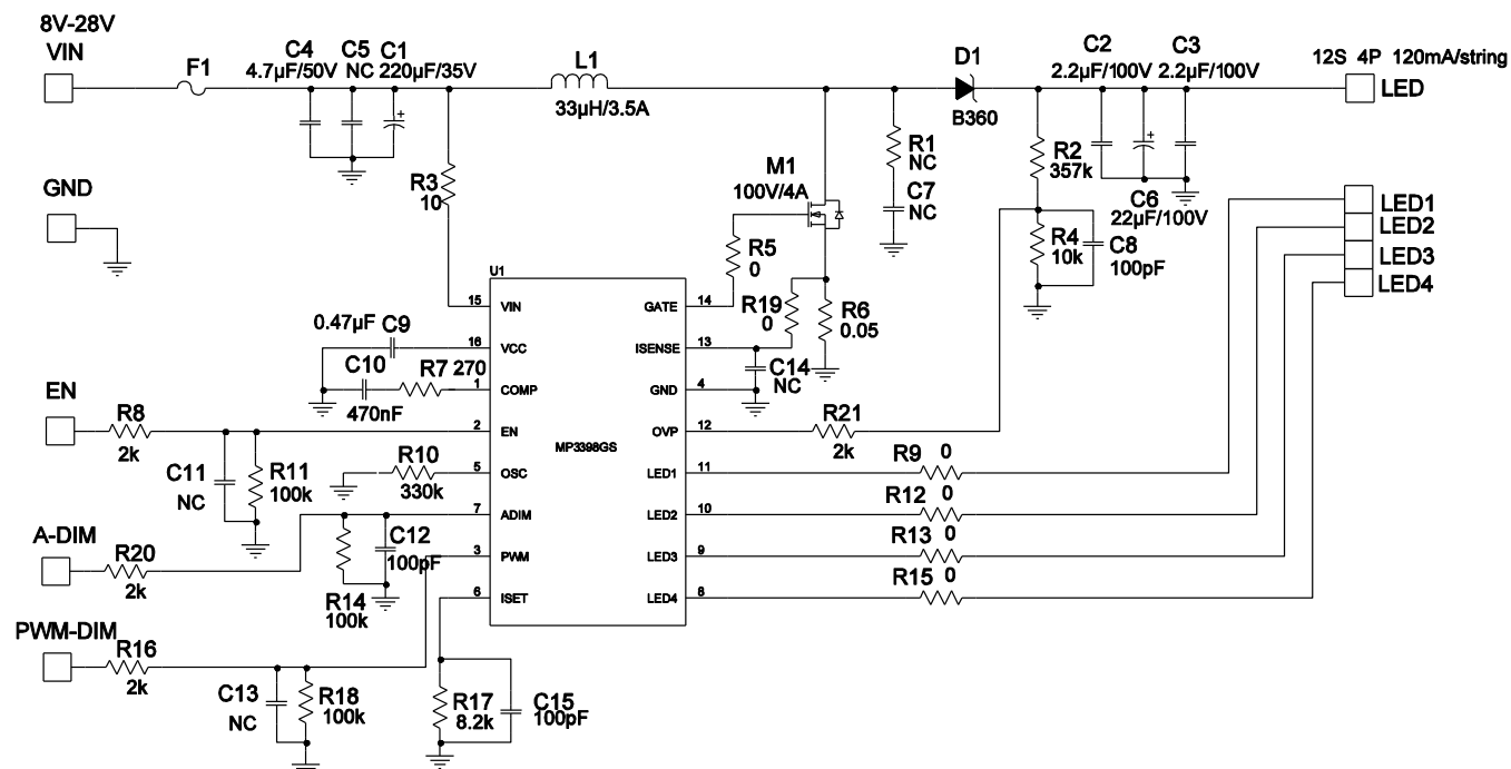
Figure 4: 4 string, 12 LED in series, 120mA/string application (Some components are reasonably adjustable based on real case)
