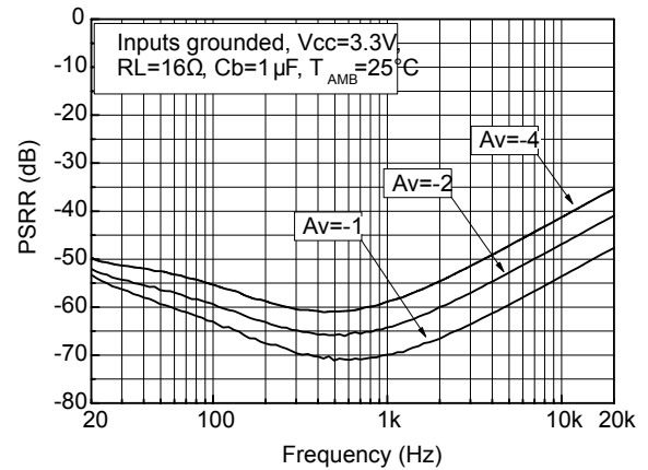
Figure 23. Power supply rejection ratio vs. frequency V_{CC} = 3.3 V
