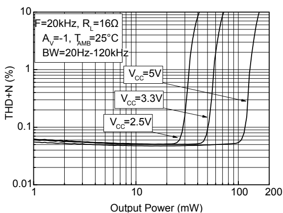
Figure 26. Total harmonic distortion plus noise vs. output power R_L = 16 \Omega , F = 20 kHz
