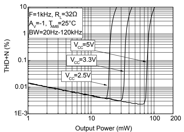
Figure 27. Total harmonic distortion plus noise vs. output power R_L = 32 \Omega , F = 1 kHz
