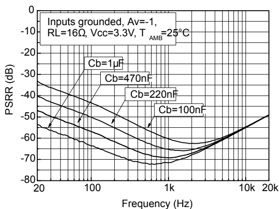
Figure 24. Power supply rejection ratio vs. frequency V_{CC} = 3.3 V , A_v = -1
