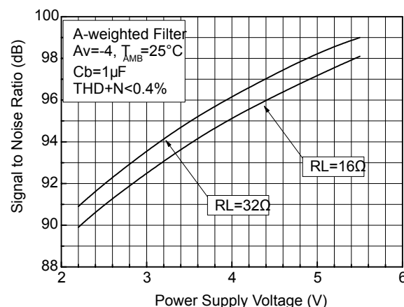
Figure 17. Signal-to-noise ratio vs. power supply voltage A weighted A_V=-4
