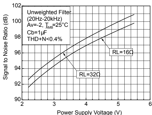
Figure 16. Signal-to-noise ratio vs. power supply voltage A unweighted A_V=-2
