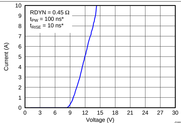
Figure 3. TLP, t_{PW} = 100 nS, t_{RISE} = 10 nS, Data to GND
