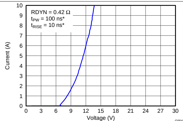
Figure 4. TLP, t_{PW} = 100 nS, t_{RISE} = 10 nS, GND to Data
