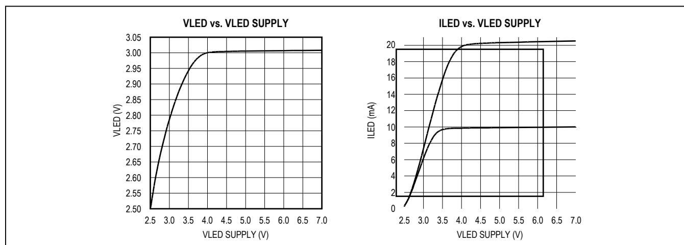
Figure 13. LED Brownout
