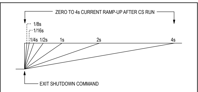
Figure 4. Ramp-Up Behavior
