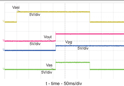
Figure 37. ASI and Delayed OUT Power-up Timing – No Input, BQ24041
