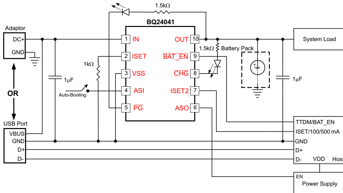
Figure 33. Typical Application Circuit: BQ24041, with ASI and ASO
