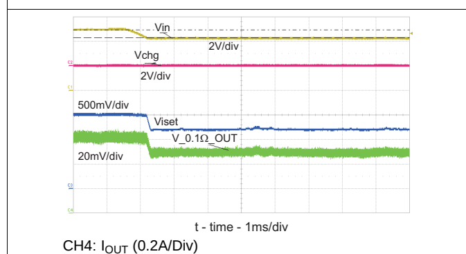
Figure 27. ISET Shorted During Normal Operation
