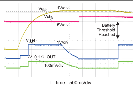
Figure 24. Battery Removal with OUT and TS Disconnect 1st, With 100 \Omega Load
