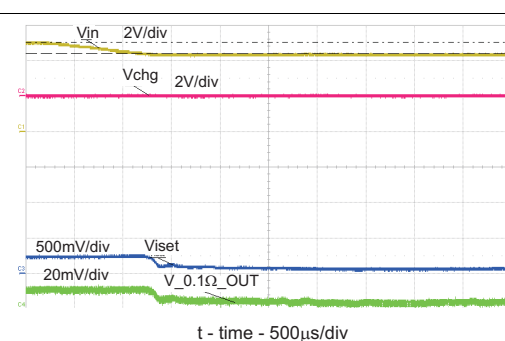
Figure 28. ISET Shorted Prior to USB Power-up
