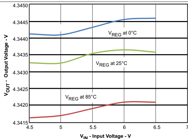
Figure 5. Line Regulation
