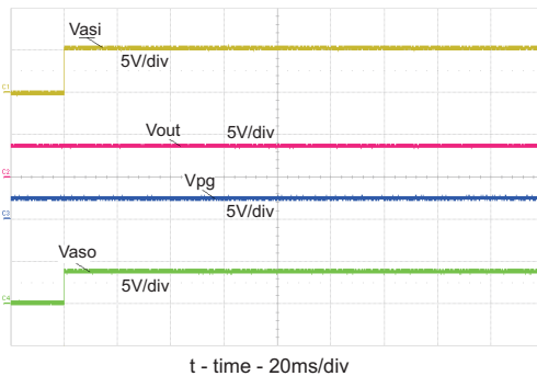
Figure 15. Power-up Timing
