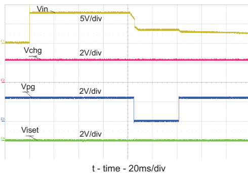
Figure 19. OVP 8V Adaptor - Hot Plug
