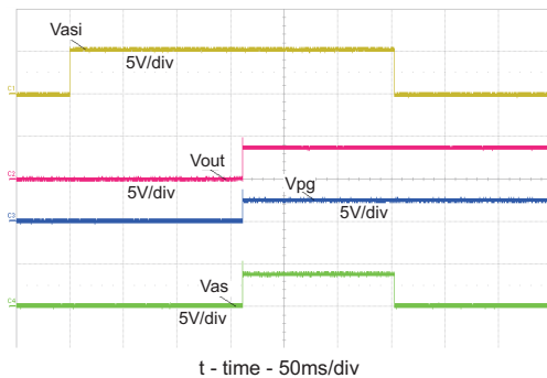
Figure 16. Power-up Timing – No Battery or Load
