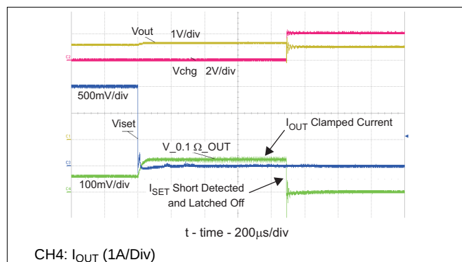
Figure 27. ISET Shorted During Normal Operation
