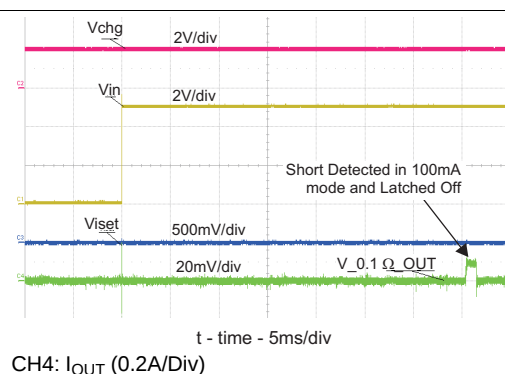
Figure 28. ISET Shorted Prior to USB Power-up
