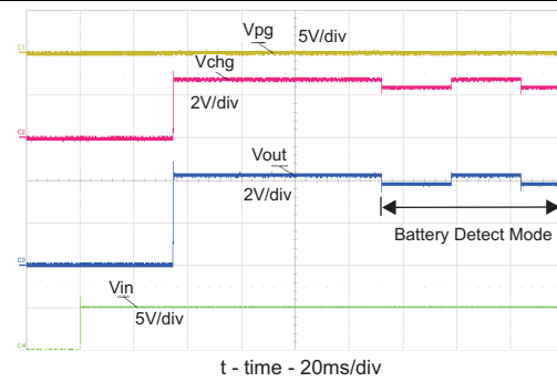
Figure 22. Hot Plug Source w/No Battery – Battery Detection
