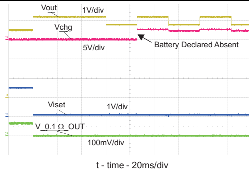
Figure 23. Battery Removal – GND Removed 1st, 42 \Omega Load
