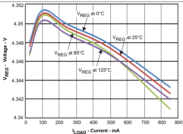
Figure 4. Load Regulation
