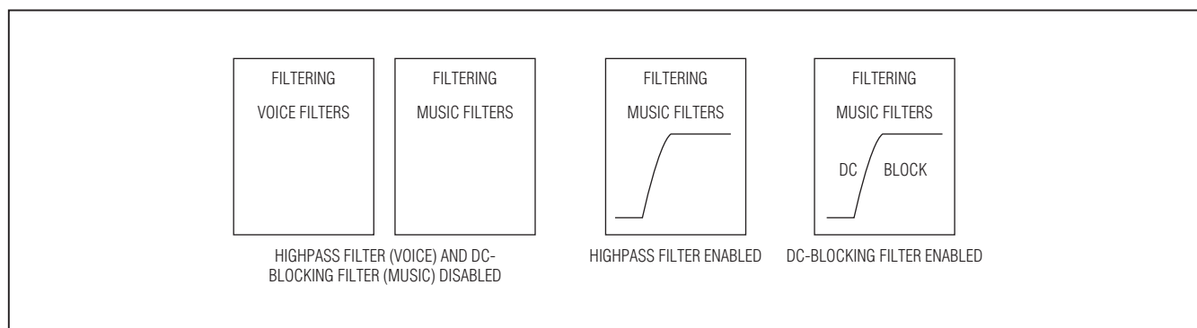
Figure 11. DAI_ Filtering Blocks
