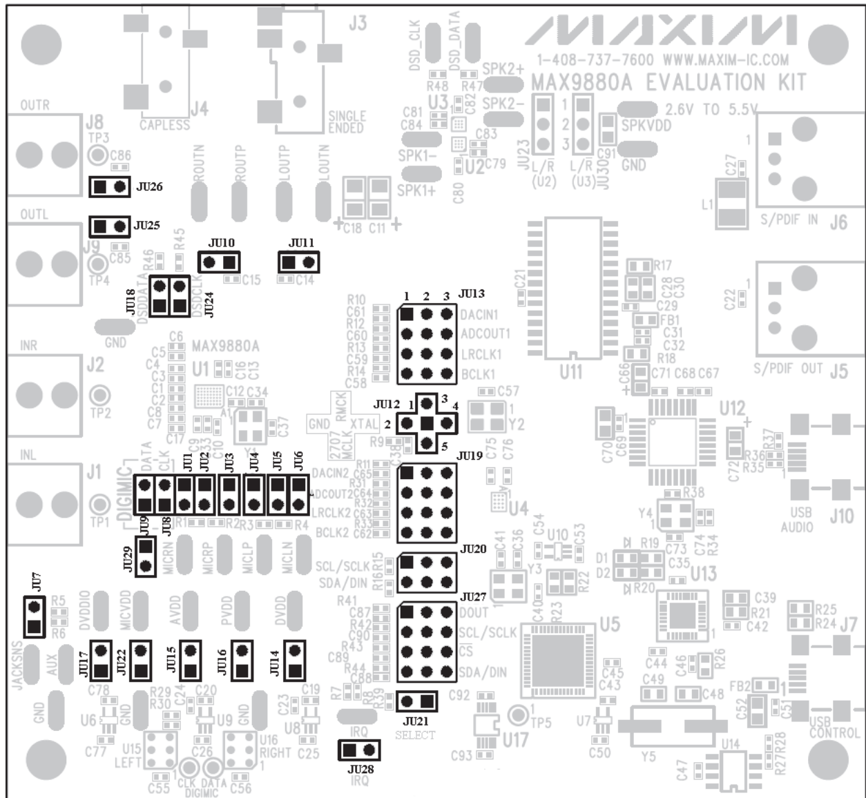
Figure 1. Default Shunt Positions (JU13, JU19, JU20, and JU27)
