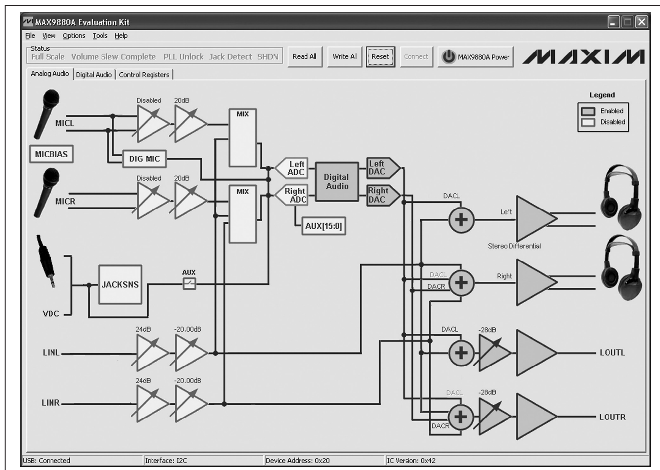
Figure 3. Analog Audio Tab
