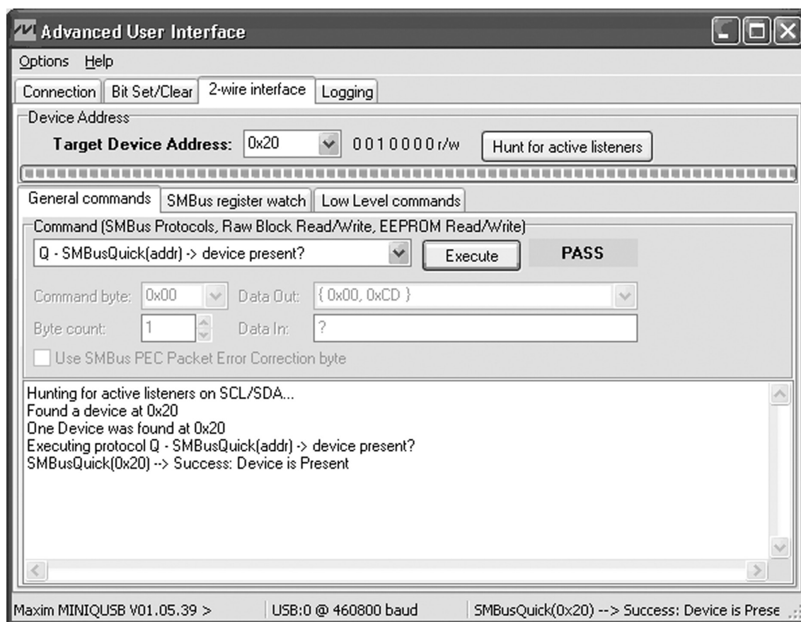
Figure 19. Advanced User Interface (2-Wire Interface Tab's General Commands Tab)
