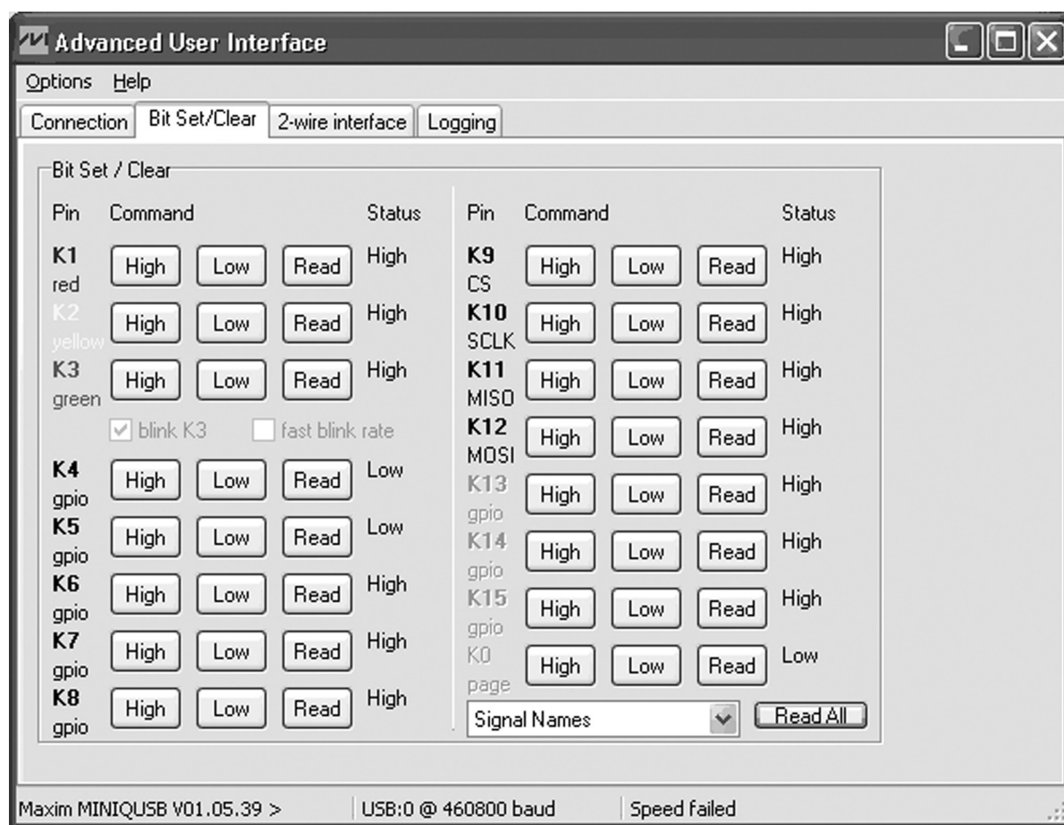
Figure 18. Advanced User Interface (Bit Set/Clear Tab)
