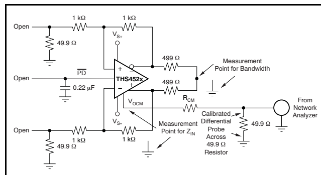
Figure 32. V_{OCM} Input Test Circuit
