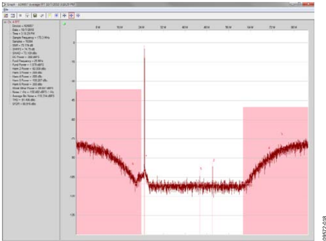
Figure 18. Graph – AD6657 Average FFT Window of VisualAnalog, NSR Enabled
