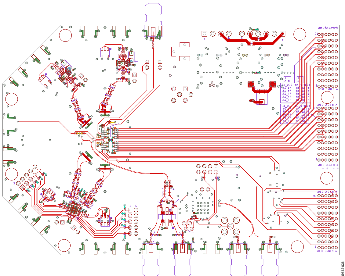
Figure 36. AD6657/AD6642 Evaluation Board, Bottom Side
